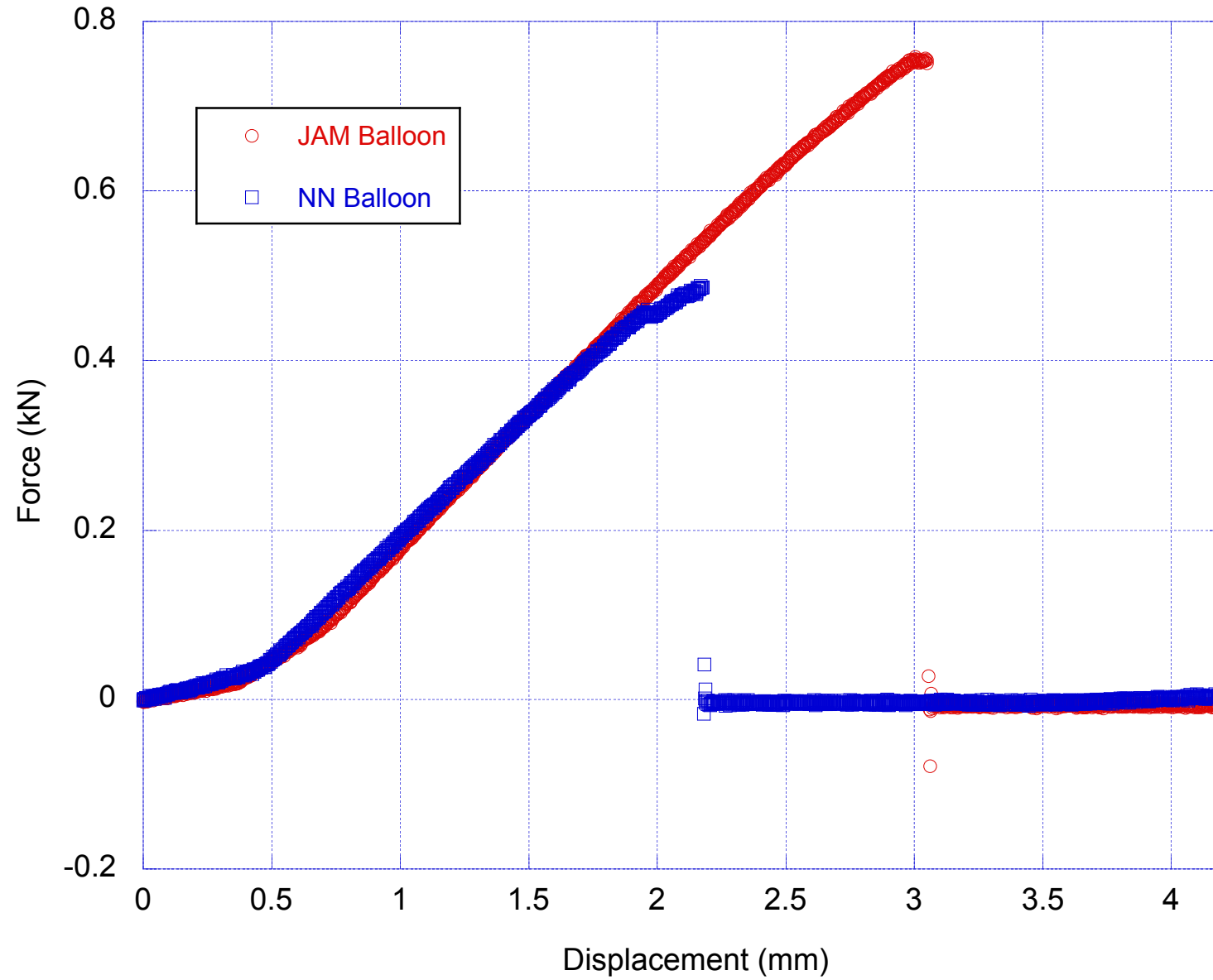
Epoxy with Glass Microspheres Data
