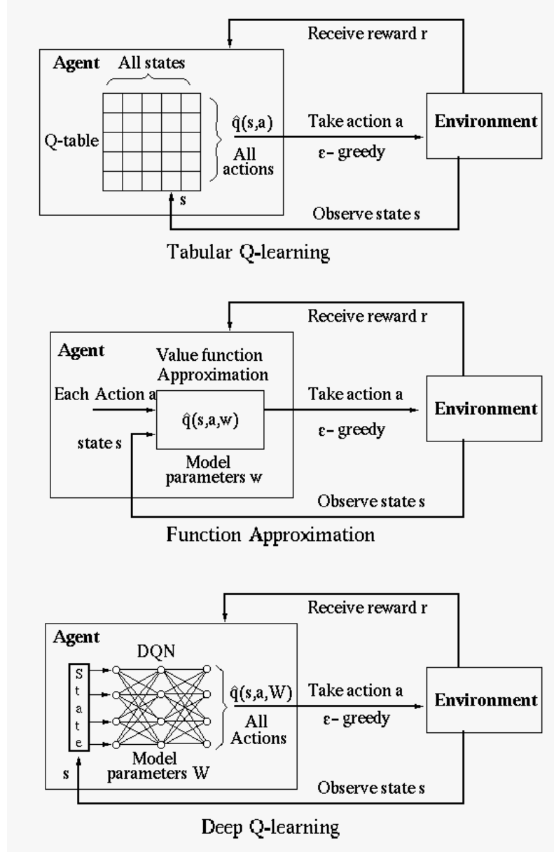
Figure 20.13 Three Q-Learning Methods: Tabular, Function Approximation, and Deep Q-Learning
