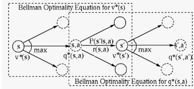
Figure 20.4 Bellman Optimality Equations for State and Action Values
