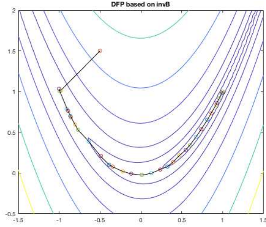
Figure 2.10 Search Path of DFP based on \mathbf{B}^{-1}
