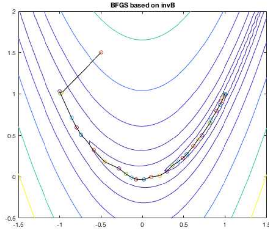
Figure 2.11 Search Path of BFGS based on \mathbf{B}^{-1}
