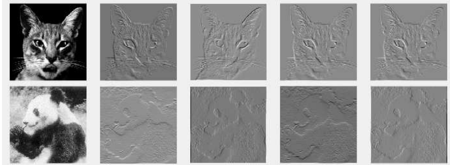
Figure 18.16 Directional Filtering
