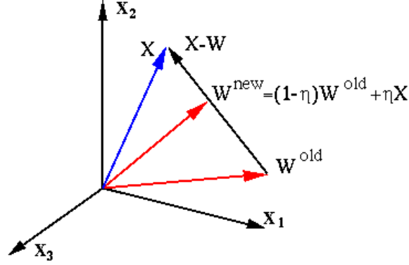
Figure 19.1 Modification of Weight Vector of the Winner
