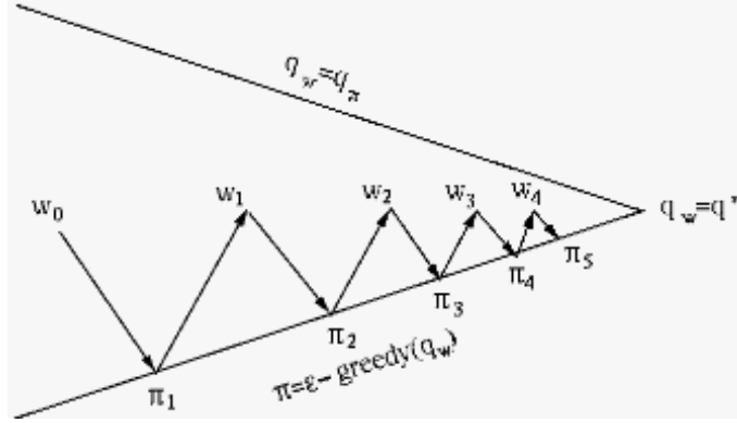
Figure 20.12 Policy Iteration Based on Approximated Value Functions
