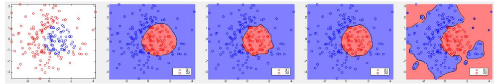
Figure 14.14 Test 3 of Kernelized Bayes Classifier
