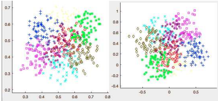
Figure 18.8 Autoencoder (left) vs. PCA (right) for Dimension Reduction for a 3-D Dataset
