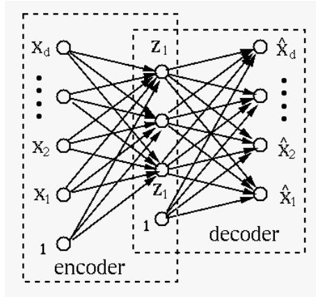
Figure 18.6 Three layer Network for Autoencoder
