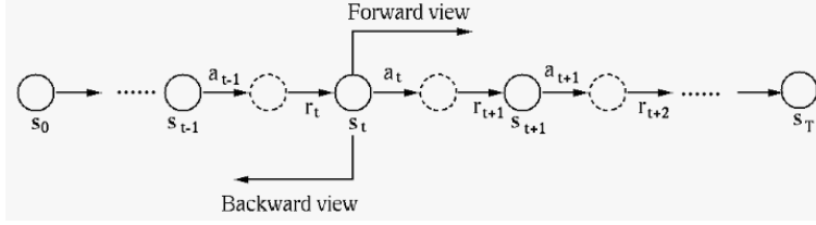
Figure 20.10 Forward View and Backward View
