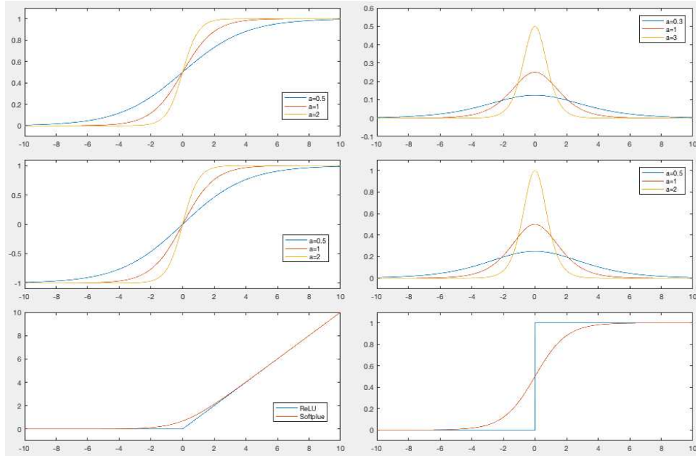
Figure 17.2 Activation Functions (left) and Their Derivatives (right) Logistic (top), Tanh (middle), and ReLU and Softplus (bottom)
