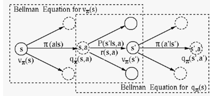
Figure 20.3 Bellman Equations for State and Action Values
