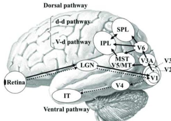
Figure 18.13 Visual Pathways
