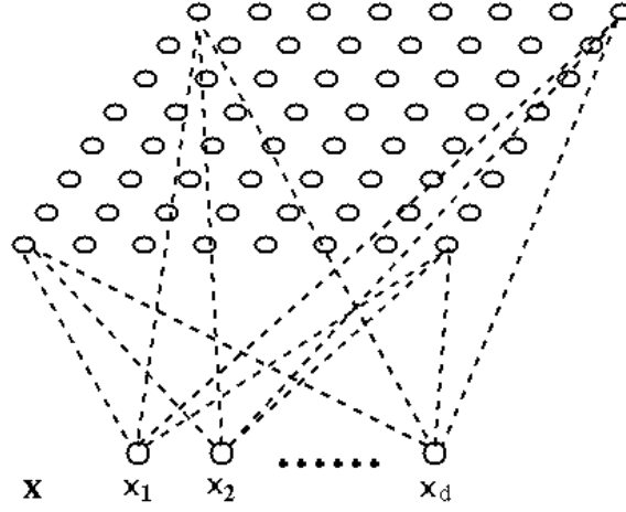
Figure 19.6 Self-Organizing Map
