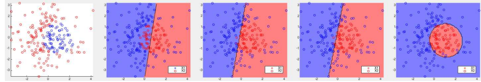
Figure 14.13 Test 2 of Kernelized Bayes Classifier
