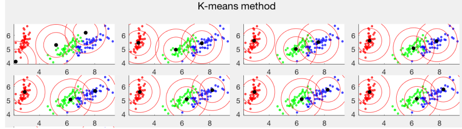
Figure 15.7 Clustering of Iris Dataset by K-Means Method
