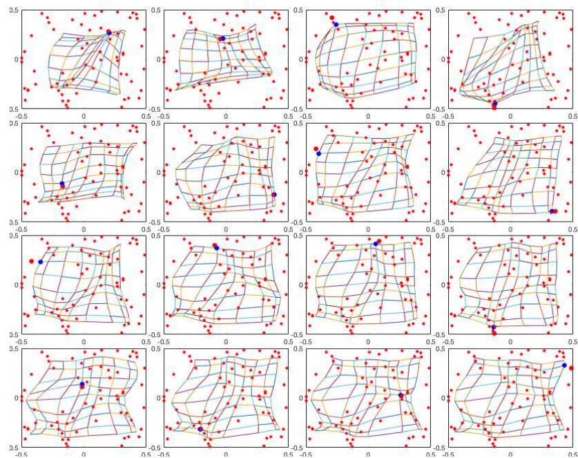
Figure 19.8 Iterative Learning of SOM (Subsequent Iterations)
