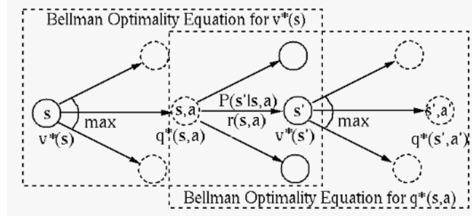
Figure 20.3 Bellman Optimality Equations for State and Action Values
