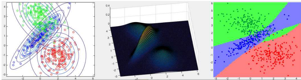
Figure 13.7 Naive Bayes Classification of Three Classes
