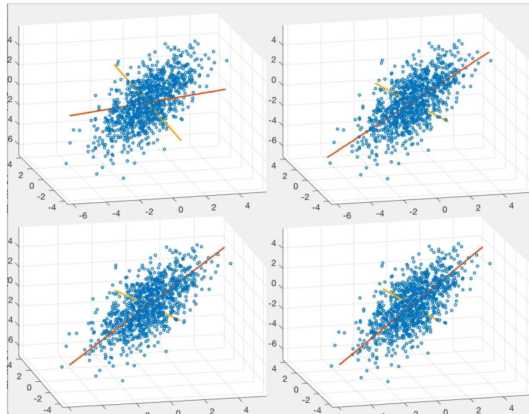
Figure 11.6 Column vectors in \mathbf{W} iteratively approach the principal directions of dataset (3-D)
