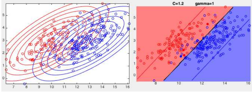
Figure 14.10 Example of Classification by SMO
