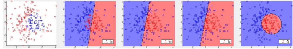
Figure 14.13 Example 2 of Kernelized Bayes Classifier
