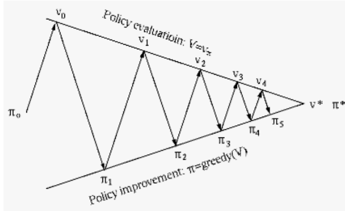
Figure 20.4 Convergence of Policy Iteration
