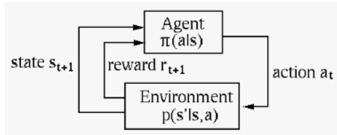
Figure 19.14 Reinforcement Learning: Agent and Its Environment
