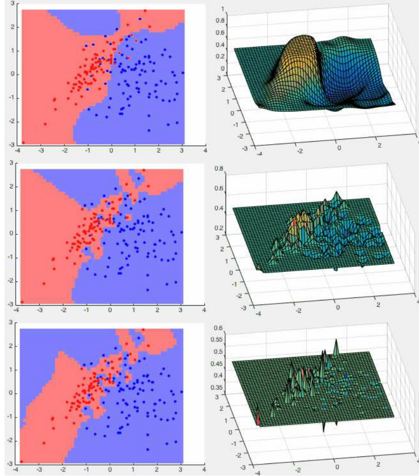
Figure 8.6 Classification Results with Different \alpha Values
