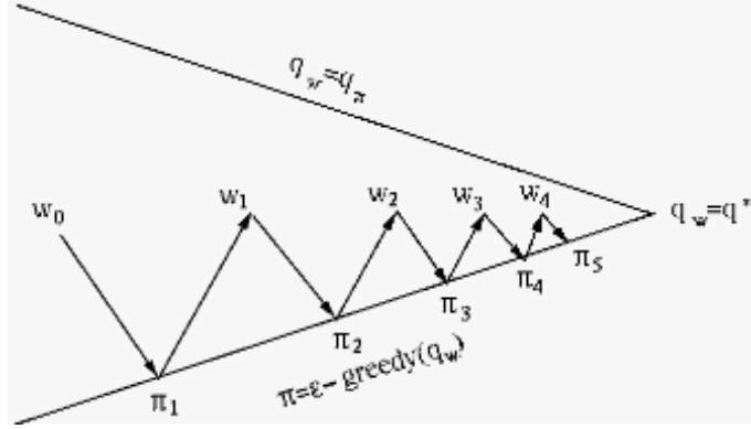
Figure 20.11 Policy Iteration Based on Approximated Value Functions
