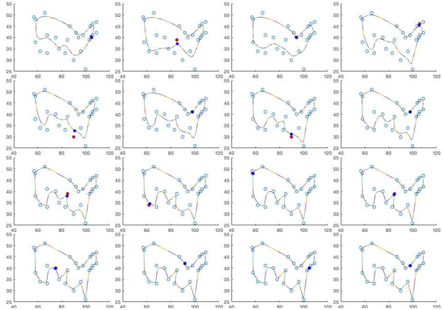
Figure 19.10 SOM Applied to the TSP (Subsequent Iterations)
