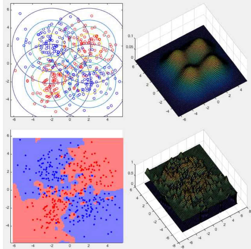
Figure 8.8 Gaussian Process Classification for the XOR Problem
