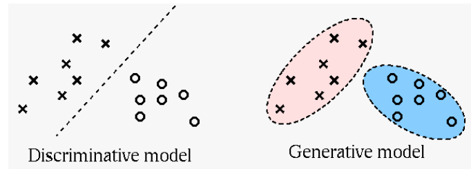
Figure 13.1 Discriminative vs. Generative Models
