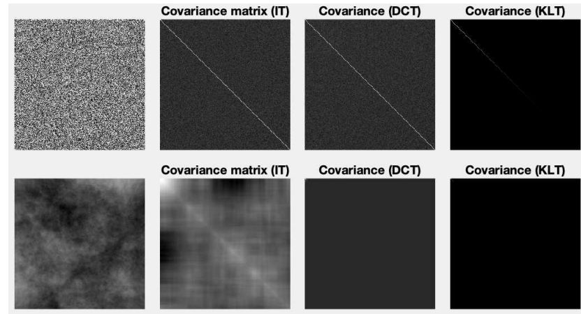
Figure 10.5 Images of Clouds and Sands
