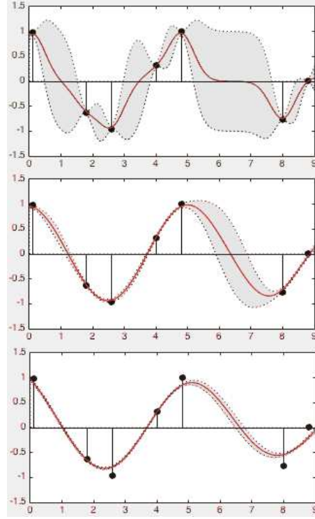
Figure 8.4 Over Fitting (top) and Under Fitting (bottom) by GPR
