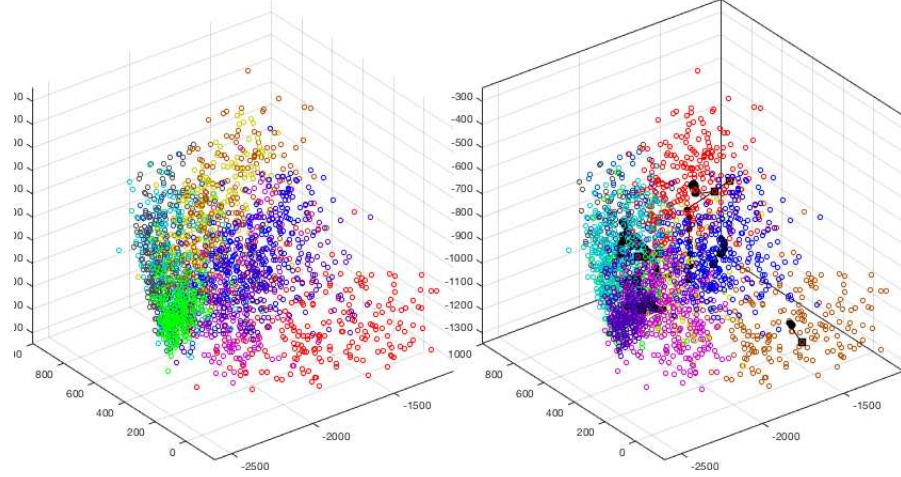
Figure 15.3 K-Means Clustering of Handwritten Digits, ground truth classes (left) vs. clusters (right)
