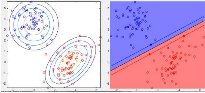
Figure 14.5 A Simple Example of Binary Classification by SVM
