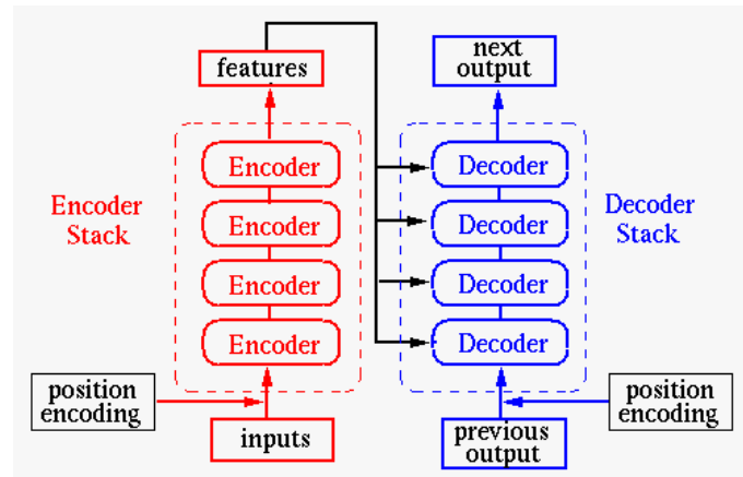
Figure 21.2 The Encoder and Decoder Stacks
