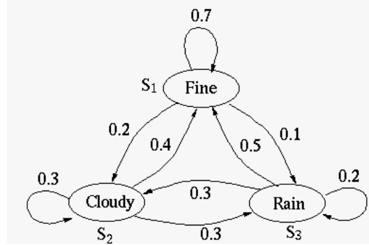
Figure 20.1 Stochastic matrix for LA Weather
