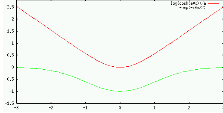
Figure 12.1 Two typical G-functions
