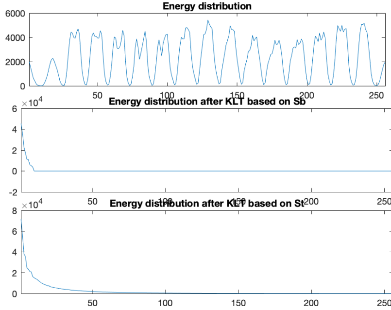
Figure 10.14 Energy distribution before (top) and after the KLT based on \mathbf{S}_B (middle), and \mathbf{S}_T (bottom)
