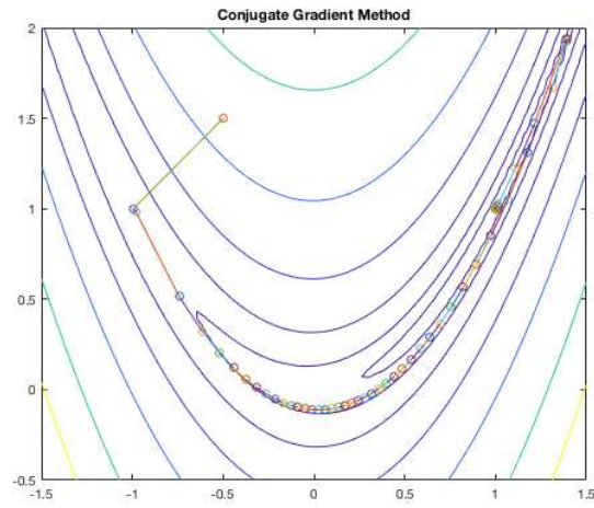
Figure 2.15 Conjugate Gradient Applied to Rosenbrock Surface
