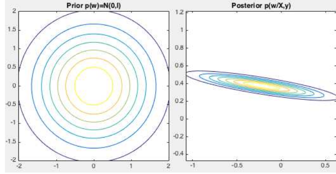
Figure 5.24 Prior and Posterior of Bayesian Regression
