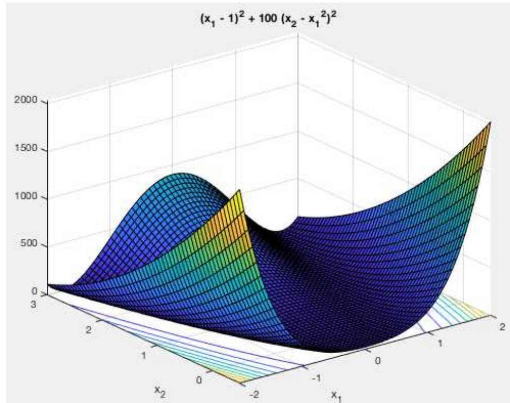
Figure 2.7 Rosenbrock Function (Left) and the Search Paths to Its Minimum (Right) The search paths for Newton's and gradient descent methods are shown in red and blue respectively.
