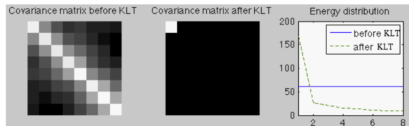
Figure 10.9 Covariance matrix before (left) and after (middle) the KLT, and energy redistribution (right)
