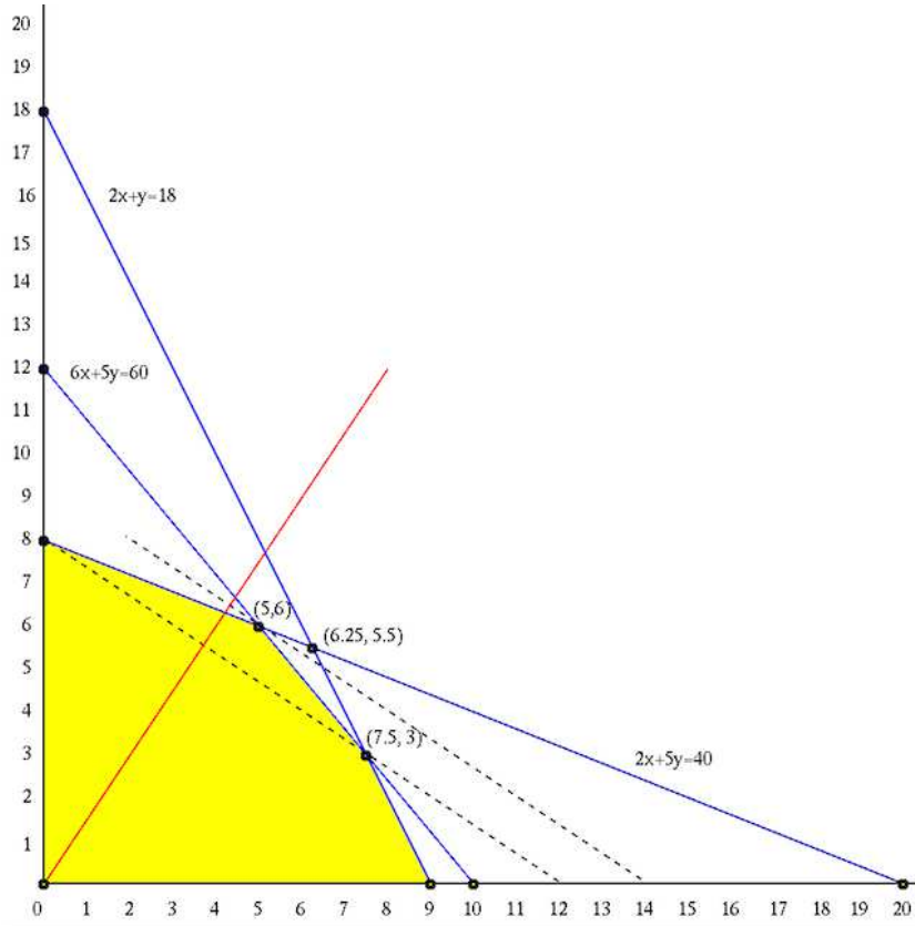
Figure 3.7 Simplex Algorithm Example (Original Problem)
