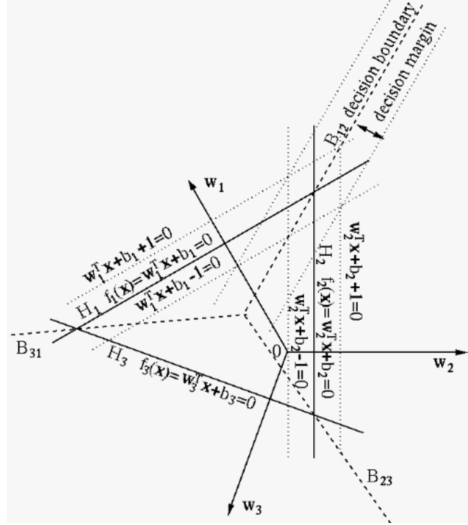
Figure 14.11 Multiclass SMV
