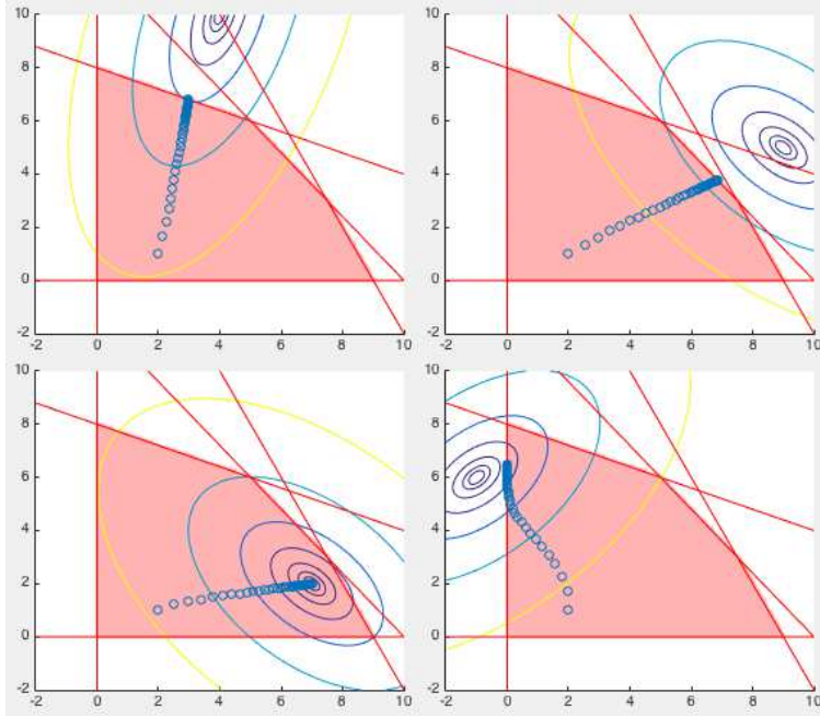
Figure 3.11 Interior Point Method for Quadratic Programming
