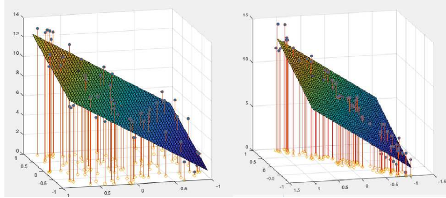
Figure 5.9 2-D Linear Regression, Well-conditioned (left) versus Ill-Conditioned (right)
