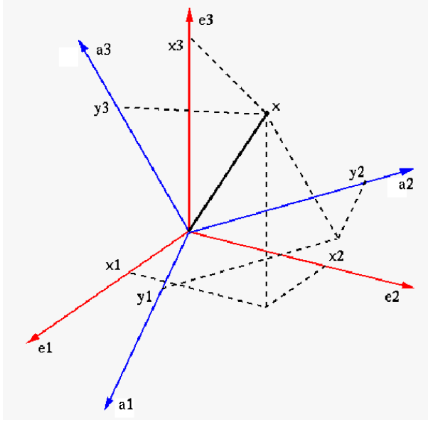
Figure 10.2 Orthogonal transform as a rotation of the coordinate system
