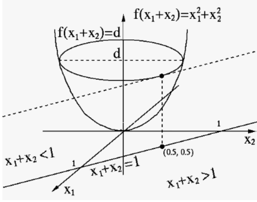
Figure 3.5 Inequality Constrained Optimization
