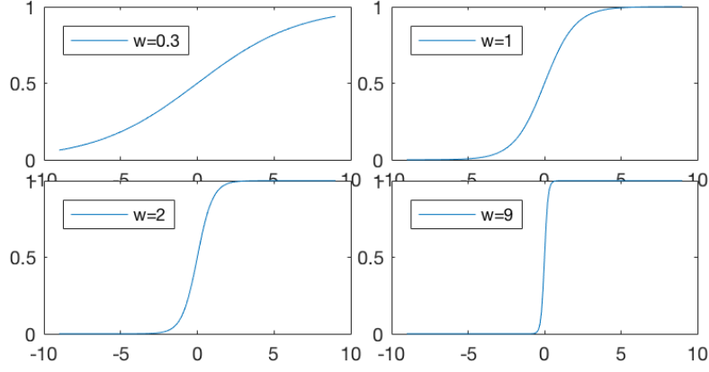
Figure 7.2 Sigmoid with Different Parameter w
