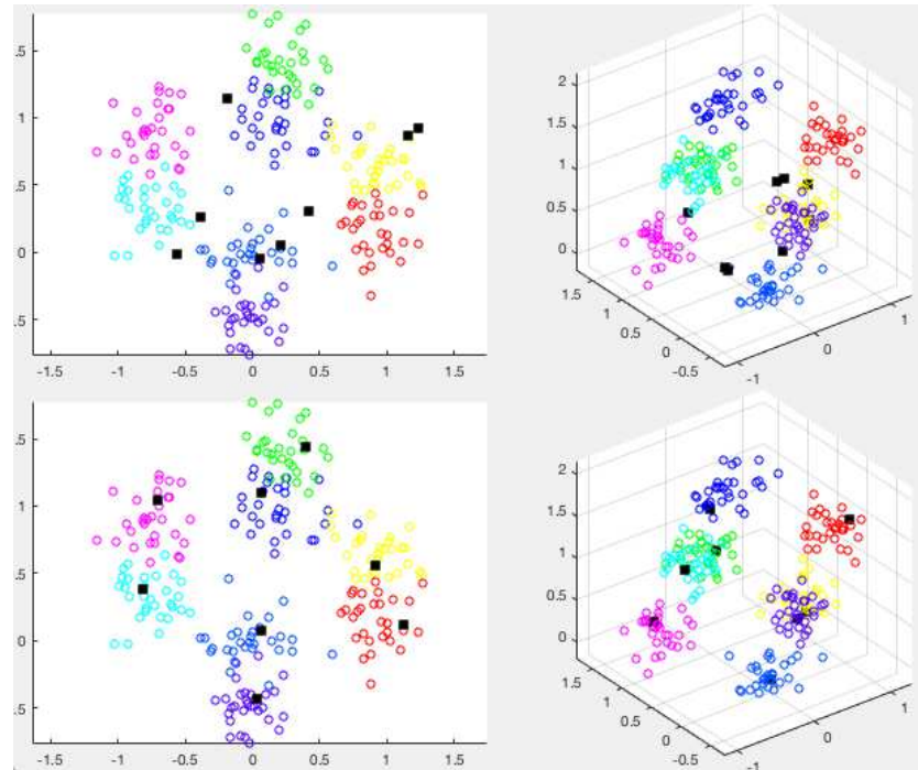
Figure 19.4 Example of Competitive Learning (3-D)
