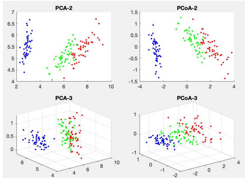
Figure 11.9 Visualization of the iris dataset based on both PCA and PCoA
