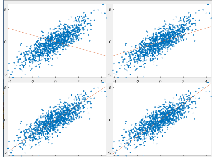
Figure 11.5 Column vectors in \mathbf{W} iteratively approach the principal directions of dataset (2-D)
