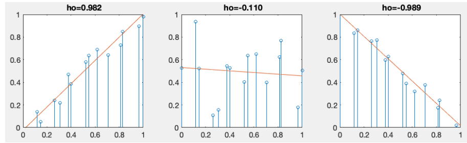
Figure 5.7 Examples of Different Correlation Coefficients
