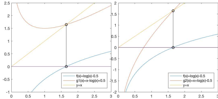
Figure 1.4 Example 1.2: Iteration converges for g(x) (left) but diverges for g'(x) (right)
