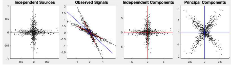
Figure 12.2 Reconstruction of independent components by ICA based on ML (2D)
