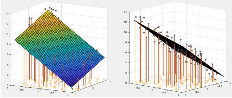
Figure 5.8 Linear Regression of a 2-D Dataset
