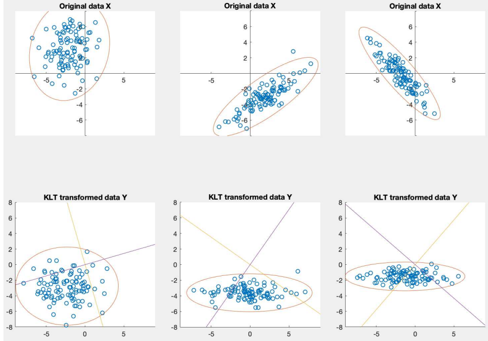
Figure 10.4 Three datasets before and after the KLT
