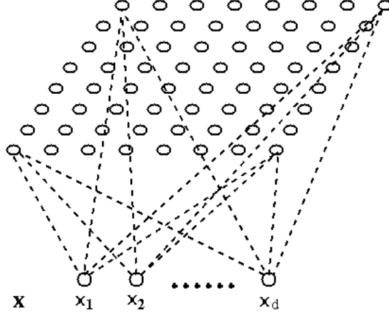
Figure 19.6 Self-Organizing Map
