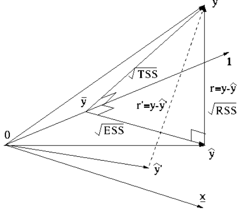
Figure 5.2 Explained, Residual and Total Sum of Squares
