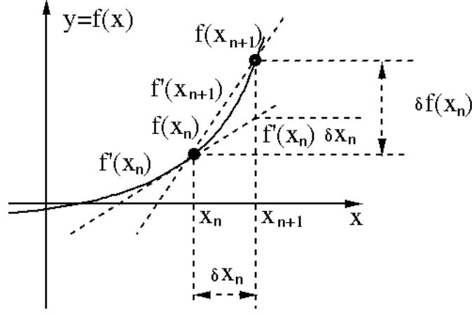
Figure 1.12 Broyden's Method (Section 1.5)
