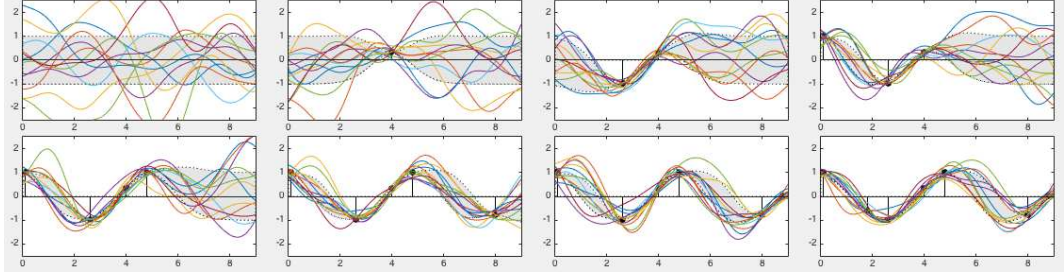
Figure 8.3 Samples Drawn from Posteriors
