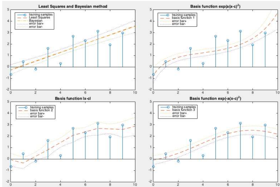
Figure 5.25 Bayesian Regression (Linear and Basis Function Based)
