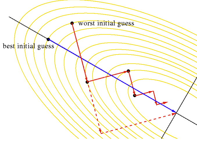
Figure 2.6 Best (blue) and Worst (red) Initial Guess
