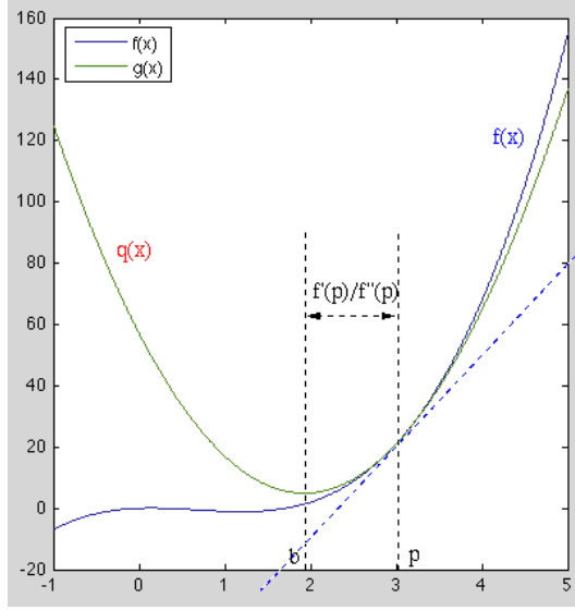
Figure 2.1 Newton's Method
