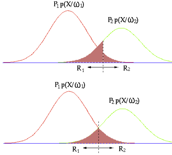
Figure 13.3 Minimum Error of Naive Bayes Classifier
