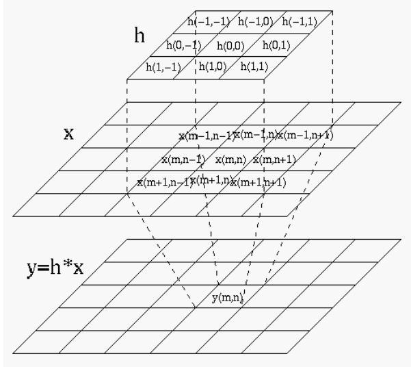
Figure 18.15 2-D Convolution
