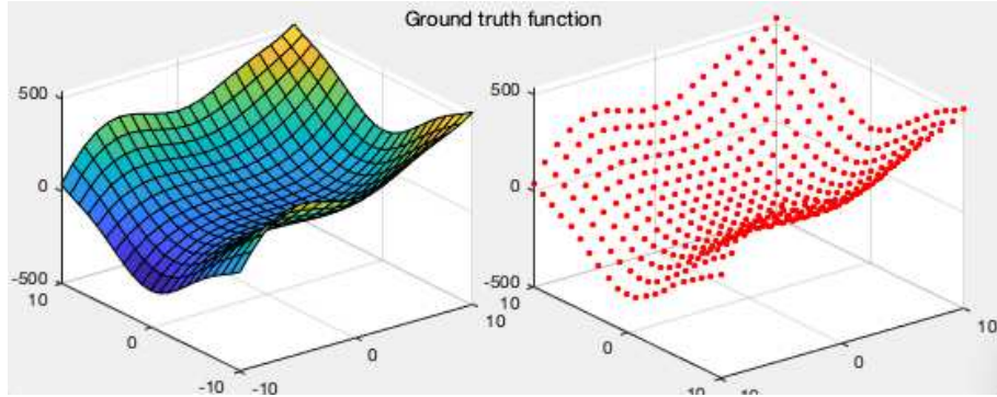
Figure 5.16 A Function and Its Samples in 2-D
