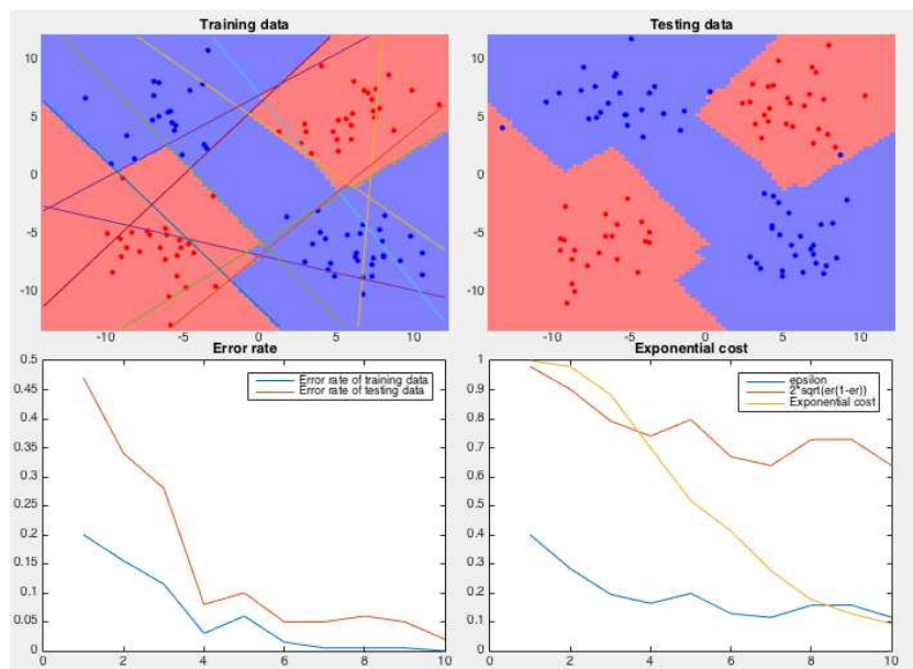
Figure 13.18 Classification of XOR Dataset (PCA method)
