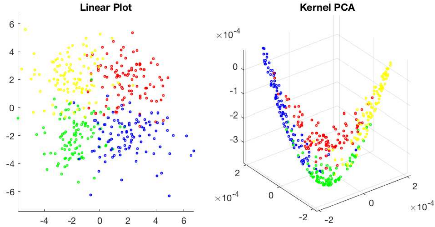
Figure 11.2 Linear and kernel PCAs for a 2-D dataset of four classes
