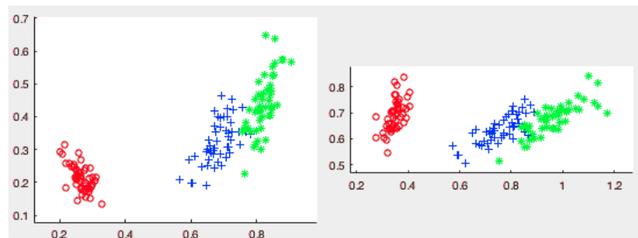
Figure 18.9 Autoencoder (left) vs. PCA (right) for Dimensionality Reduction for Iris dataset
