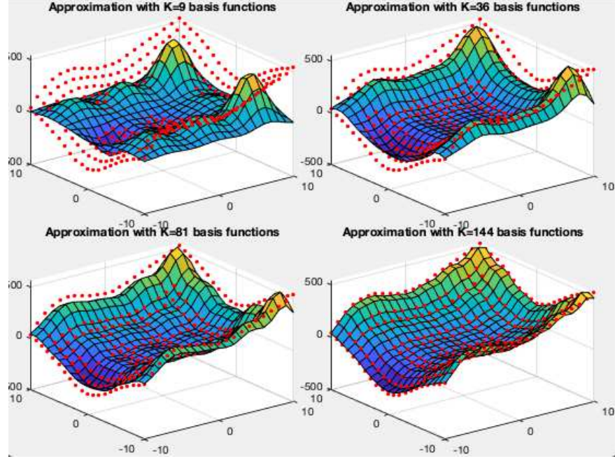
Figure 5.18 Regression Results based on Different Number of Basis Functions
