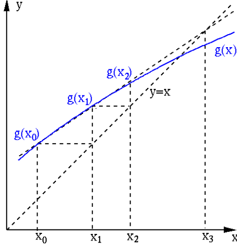
Figure 1.9 Aitken's Method
