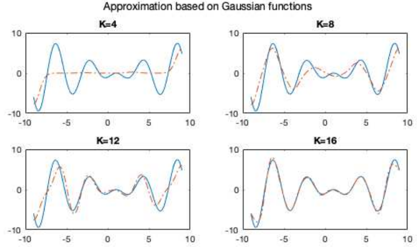
Figure 5.14 Regression based on Gaussian Basis
