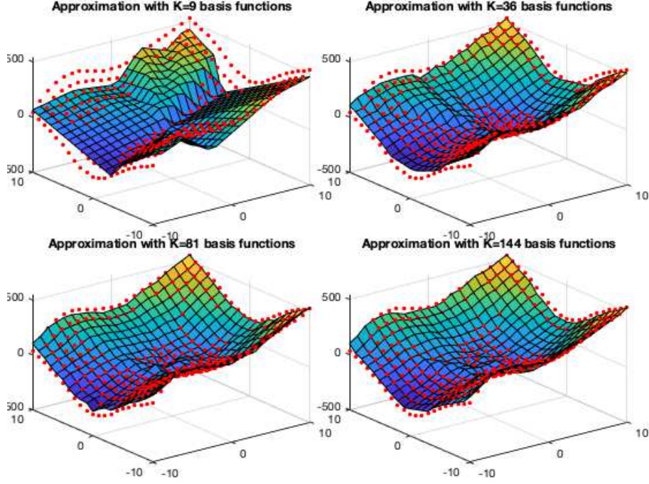
Figure 5.23 Regression based on ReLU Basis
