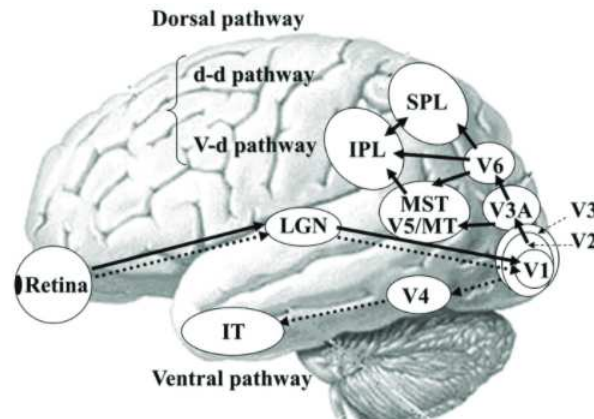
Figure 18.13 Visual Pathways
