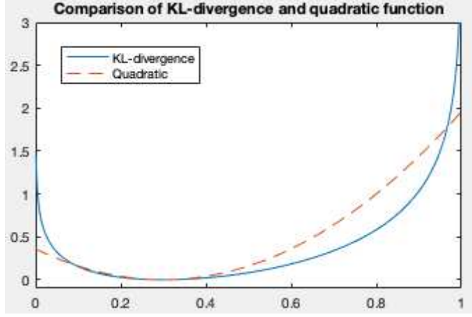
Figure 18.7 Comparison of KL-divergence and Quadratic Function
