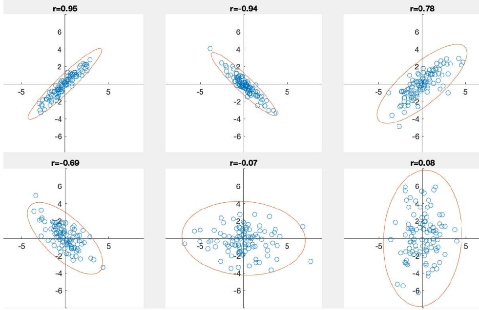
Figure 10.1 Normally distributed datasets with different covariance matrices
