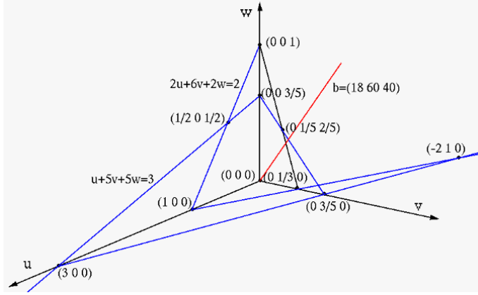
Figure 3.8 Simplex Algorithm Example (Dual Problem)
