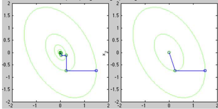
Figure 2.14 Gradient (left) vs. Conjugate Gradient (right)
