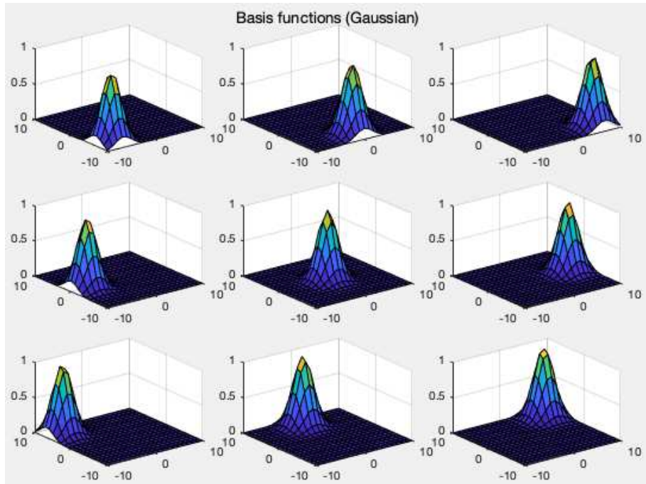
Figure 5.17 Gaussian Basis in 2-D
