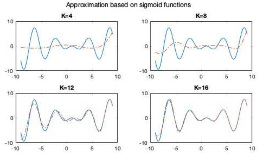
Figure 5.15 Regression based on Sigmoid Basis
