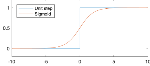
Figure 7.1 Unit Step vs. Sigmoid
