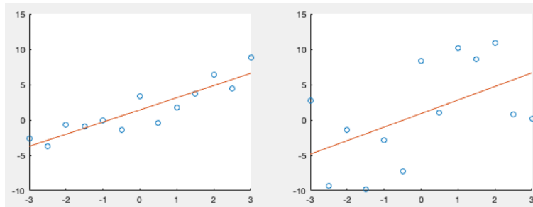
Figure 5.5 Linear Regressions with Different R^2 and \rho
