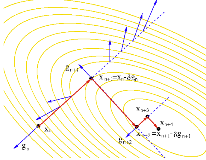
Figure 2.5 Iterations of the Gradient Descent Method
