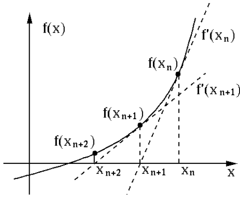
Figure 1.10 Newton-Raphson Method
