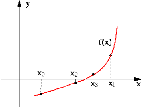
Figure 1.2 Bisection Search
