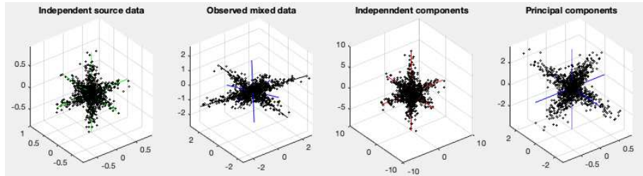
Figure 12.3 Reconstruction of independent components by ICA based on ML (3D)
