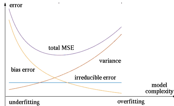
Figure 4.3 Under vs. Overfitting
