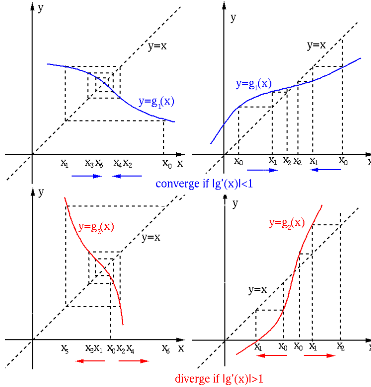
Figure 1.6 Convergence (top) and Divergence (bottom) of the Fixed Point Method
