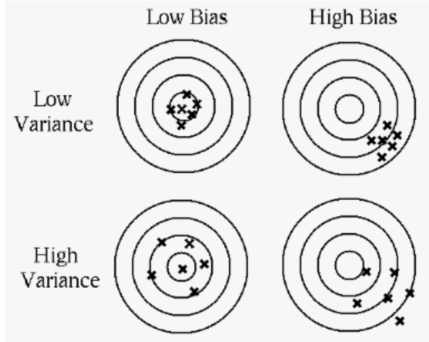
Figure 4.2 Bias-Variance Tradeoff
