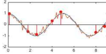
Figure 8.1 A Noisy Sinusoid
