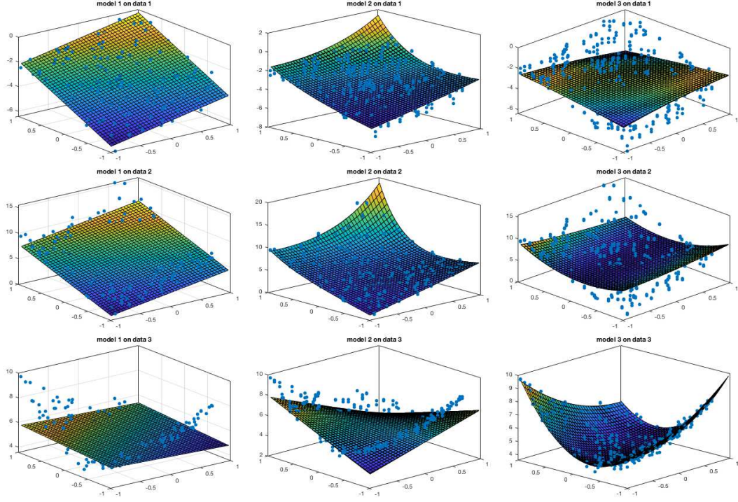
Figure 6.2 Nonlinear Regression with Multiple Datasets and Models (2-D)
