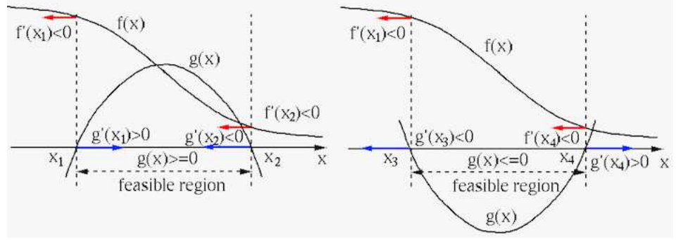
Figure 3.4 Determination of Signs of Lagrange Multipliers
