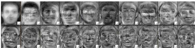
Figure 10.11 The eigen-faces
