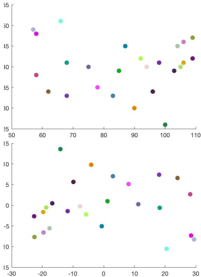
Figure 11.8 Reconstruction of the locations of north America cities by the MDS
