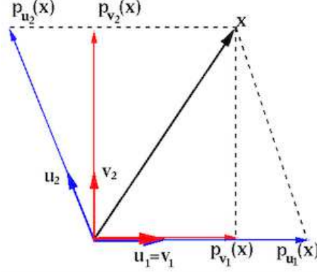
Figure 2.12 A-Orthogonality based on Matrix \mathbf{A}
