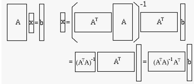
Figure 1.1 The Pseudo Inverse (Section 1.1)
