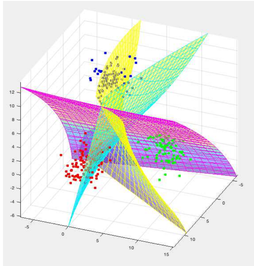
Figure 13.8 Partitioning of a 3-D Space by Quadratic Decision Boundaries
