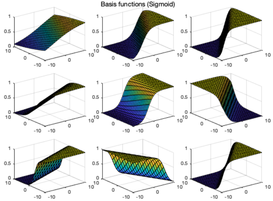
Figure 5.20 Sigmoid Basis for 2-D Regression
