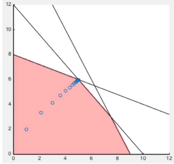
Figure 3.10 Interior Point Method for Linear Programming
