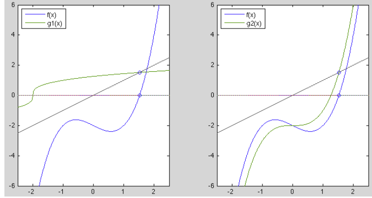
Figure 1.7 Example 1.4, plots of g_1(x) (left) and g_2(x) (right)
