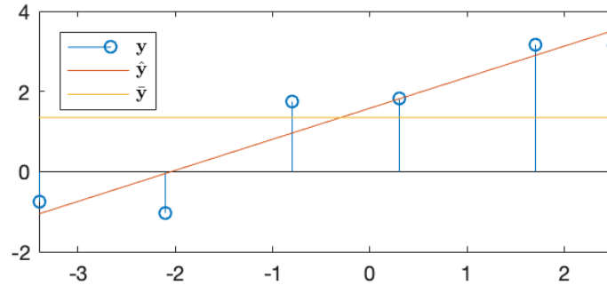
Figure 5.4 Linear Regression Example
