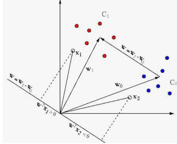
Figure 7.4 Softmax Classification
