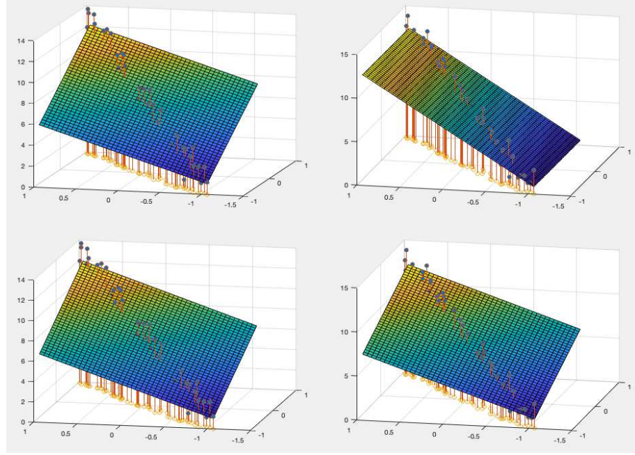
Figure 5.10 Unstable Results Generated by Regression applied to Ill-Conditioned Dataset (top) and Stable Results Generated by Ridge Regression (bottom)
