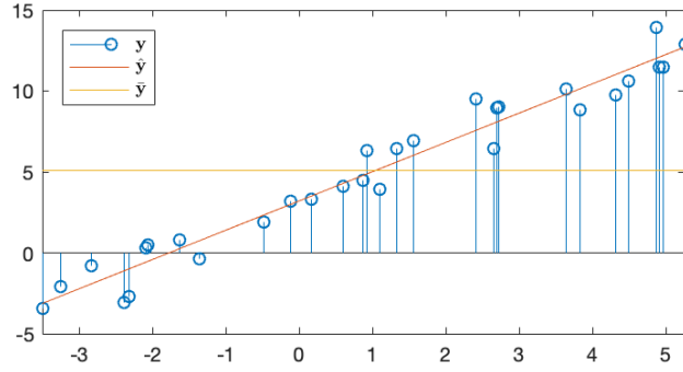
Figure 5.6 Example Showing y , \hat{y} and \bar{y}
