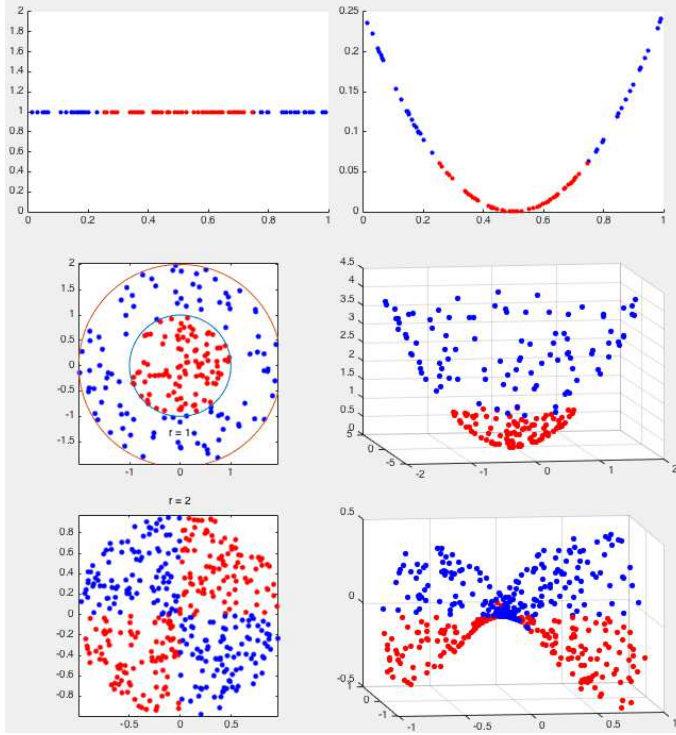
Figure 11.1 Examples of kernel mapping
