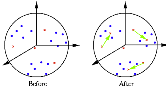
Figure 19.2 Weight Vectors Moving toward Centers of Clusters
