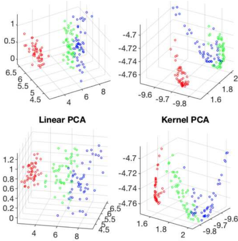
Figure 11.4 Linear and kernel PCAs for the iris dataset
