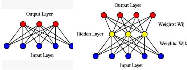
Figure 17.3 Artificial Neural Networks of Two (left) or Three (right) Layers
