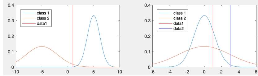
Figure 13.2 Binary Classification in 1-D
