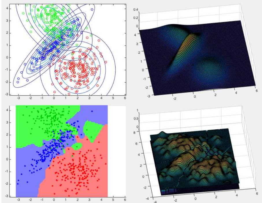
Figure 8.7 Gaussian Process for Classification (Multi-Class)
