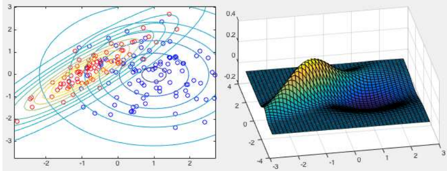
Figure 8.5 Gaussian Process for Classification (Binary)
