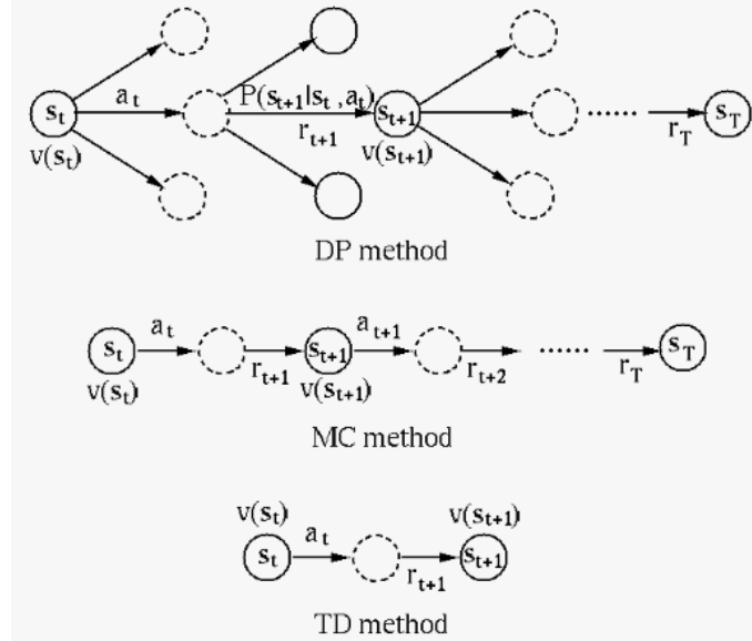
Figure 20.7 Comparison of DP, MC and TD Methods
