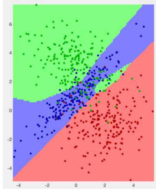
Figure 18.5 BP Network Classification of a Three-Class Dataset
