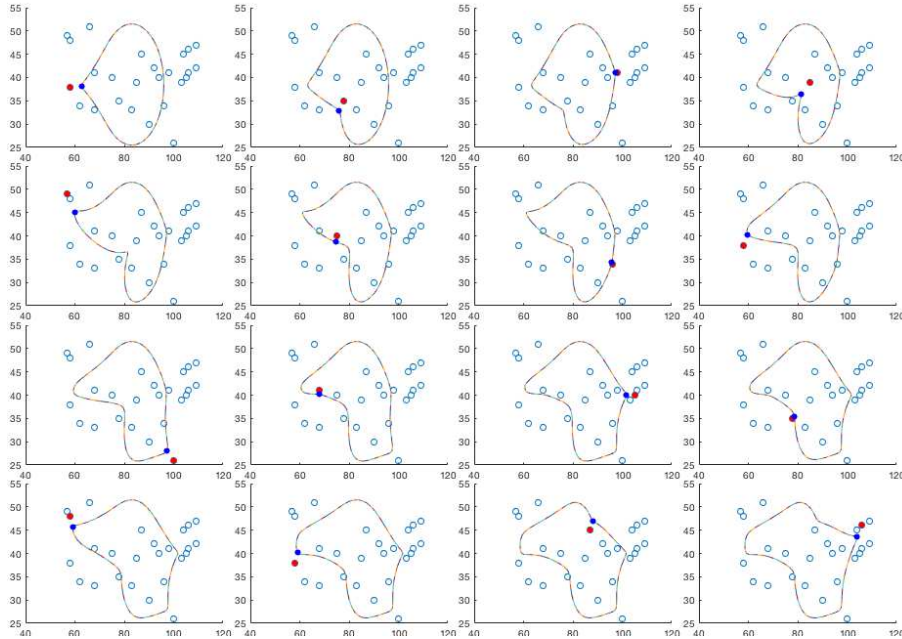
Figure 19.9 SOM Applied to the TSP (First 16 Iterations)
