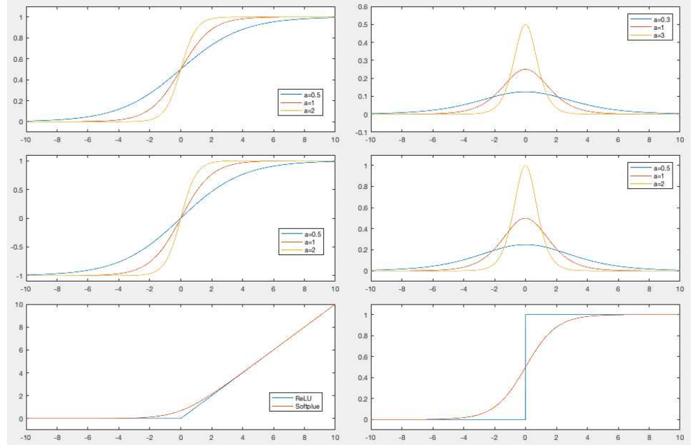
Figure 17.2 Activation Functions (left) and Their Derivatives (right) Logistic (top), Tanh (middle), and ReLU and Softplus (bottom)
