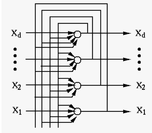
Figure 17.4 The Hopfield Network
