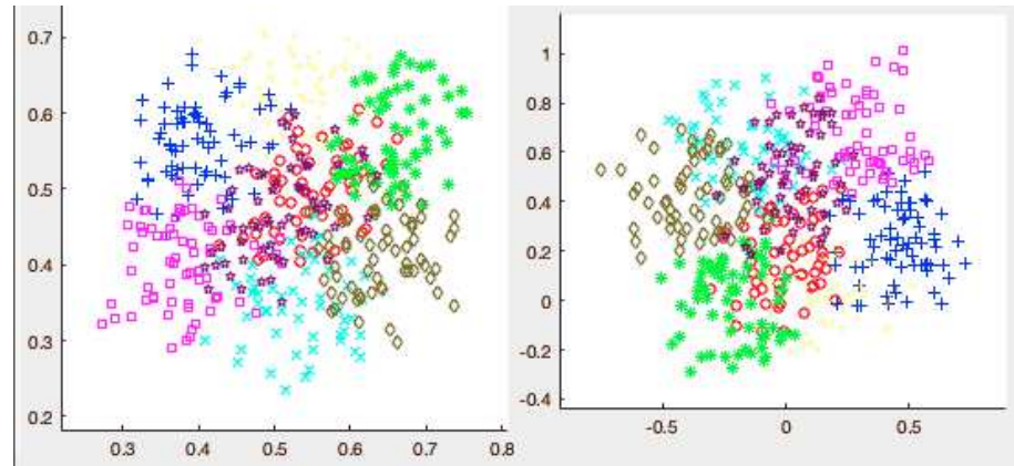
Figure 18.8 Autoencoder (left) vs. PCA (right) for Dimension Reduction for a 3-D Dataset
