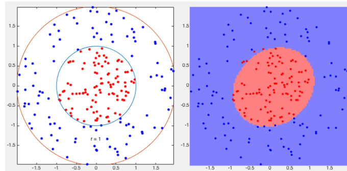
Figure 13.5 Naive Bayes Classification of Concentric Binary Classes
