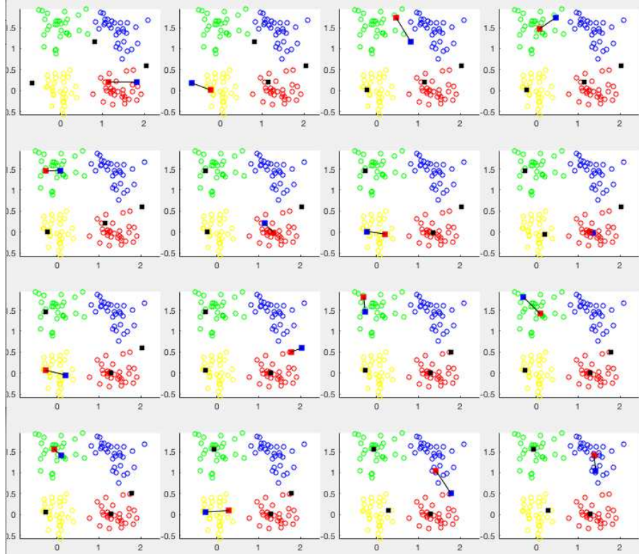
Figure 19.3 Iterative Learning of Competitive Network (2-D)
