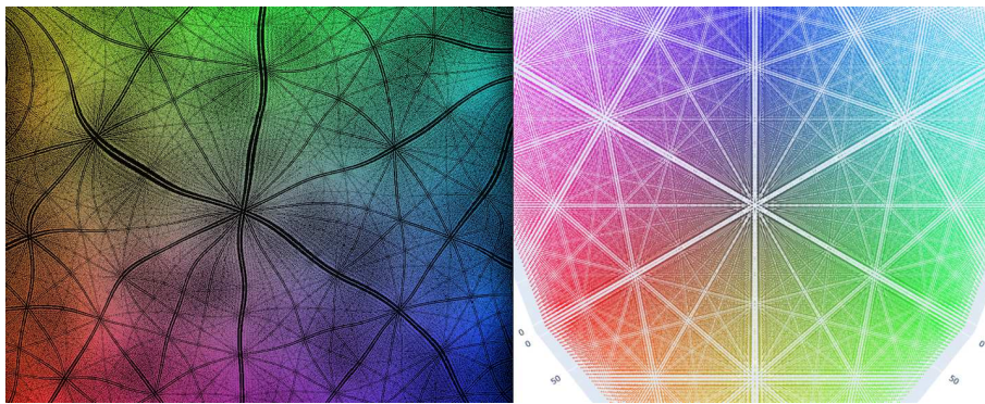
Figure 19.12 Emergent Patterns in SOM (left) and Perspective Projection of the Color Grid (right)
