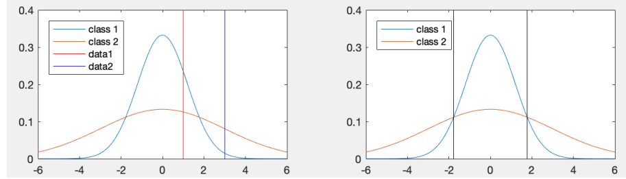
Figure 13.4 Binary Classification in 1-D Revisited
