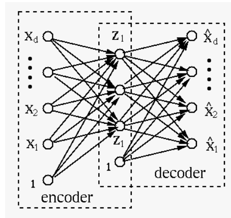
Figure 18.6 Three layer Network for Autoencoder
