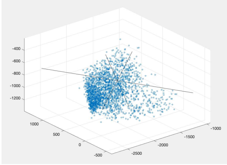
Figure 11.7 First three components of the handwritten digits dataset by the PPCA
