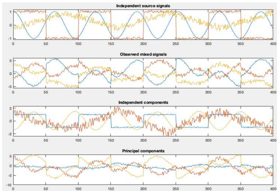
Figure 12.4 Reconstruction of independent components in time signals by FastICA
