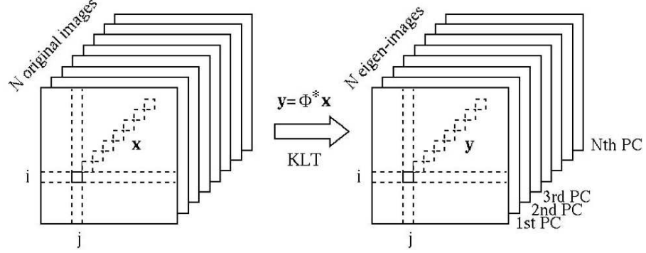
Figure 10.7 The KLT of a set of images
