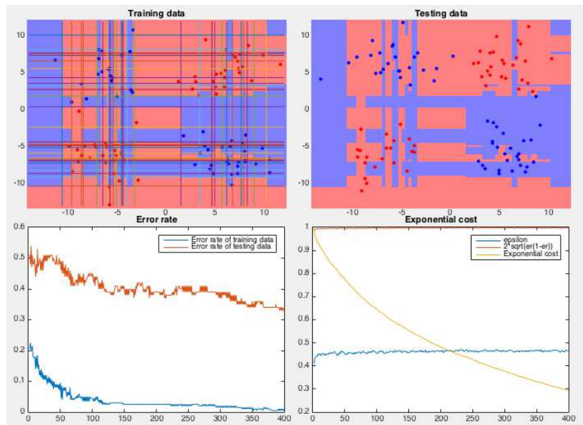
Figure 13.17 Classification of XOR Dataset (Coordinate Descent)
