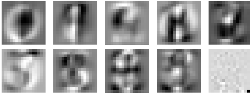
Figure 10.15 The first ten Eigen-digits
