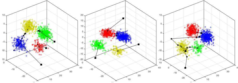
Figure 15.2 K-Means Clustering with Merge and Split
