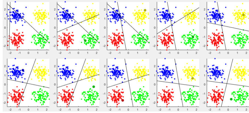
Figure 18.1 Classification by Perceptron (2-D)
