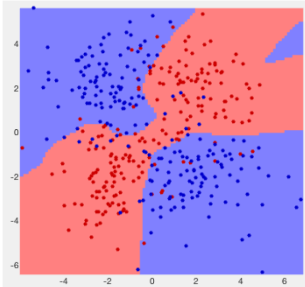
Figure 18.4 BP Network Classification of the XOR Dataset
