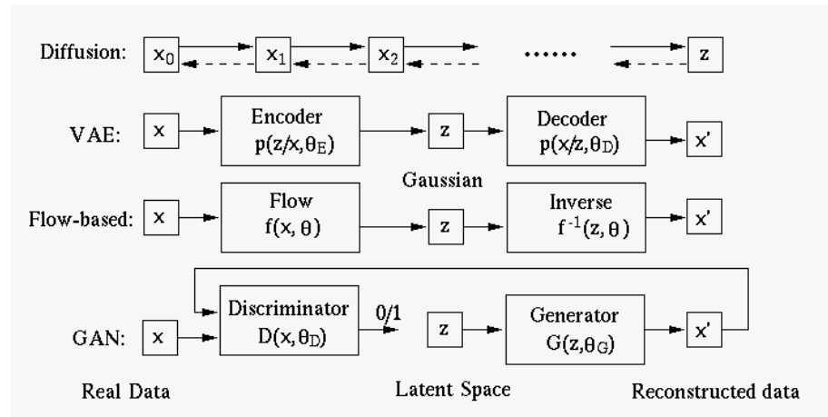
Figure 21.3 Four Generative Models
