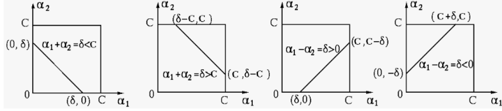
Figure 14.6 Four Cases while Updating \alpha_i and \alpha_j
