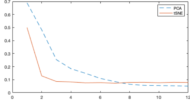
Figure 13.12 Comparison of KLT and tSNE for Feature Selection
