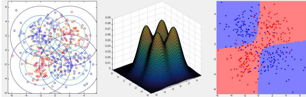
Figure 13.6 Naive Bayes Classification of XOR Binary Classes
