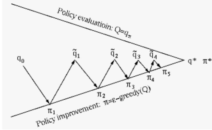
Figure 20.5 Convergence of General Policy Iteration
