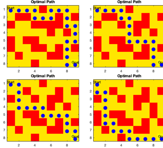
Figure 20.8 Optimal paths in four different mazes
