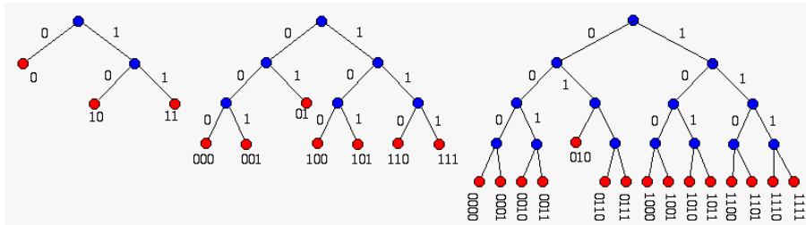
Figure 16.3 Tree Structures with 3, 7 and 15 Leaf Nodes Each for a Cluster
