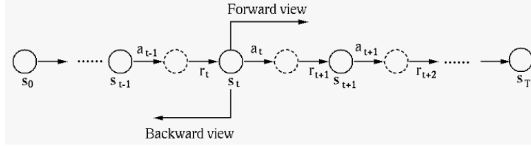
Figure 20.9 Forward View and Backward View
