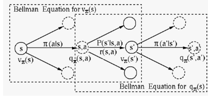
Figure 20.2 Bellman Equations for State and Action Values
