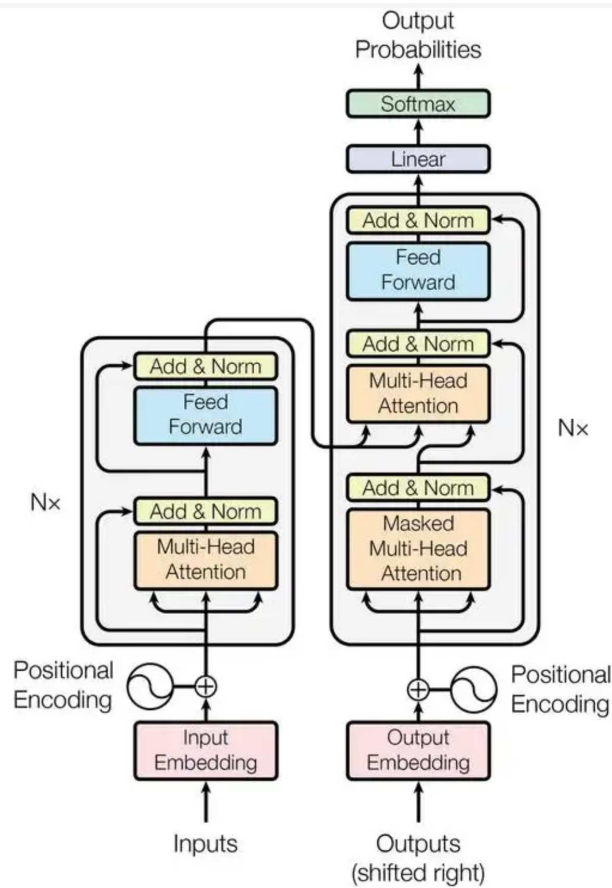
Figure 21.1 The Transformer Architecture
