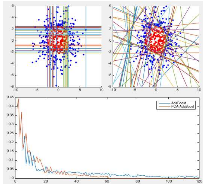
Figure 13.15 AdaBoost Classification Along Basis Vectors and PCA Directions
