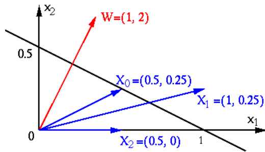
Figure 14.4 Decision Plane and Support Vectors
