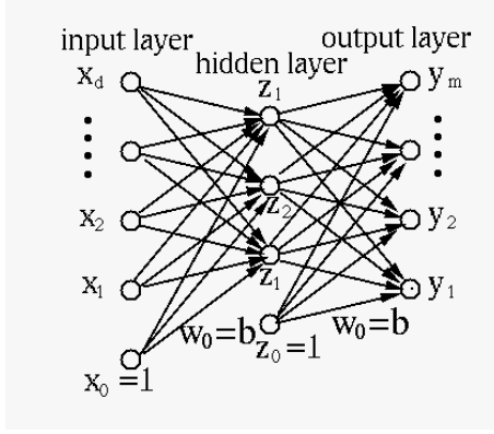
Figure 18.3 Back Propagation Network
