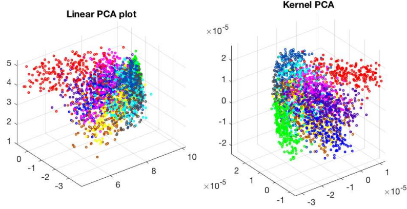
Figure 11.3 Linear and kernel PCAs for the 256-D handwritten digits
