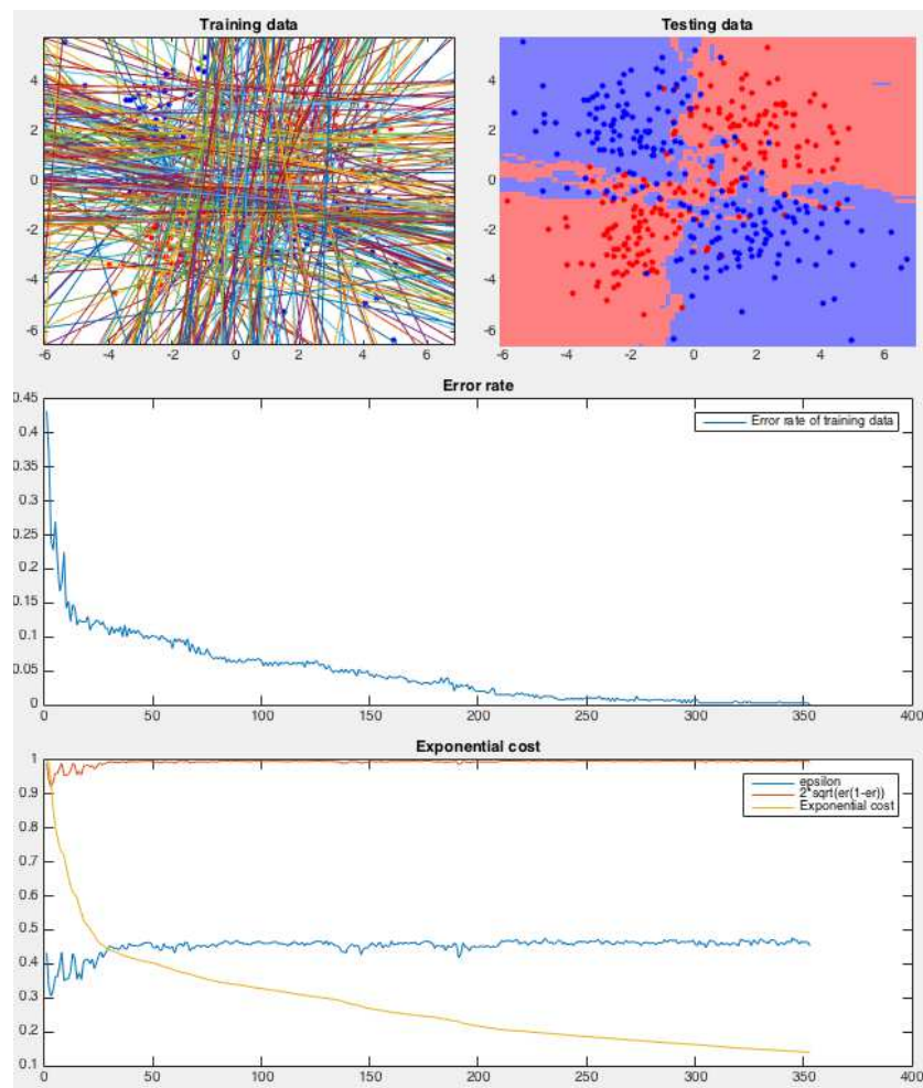
Figure 13.14 Classification by AdaBoost on XOR Dataset (final result)
