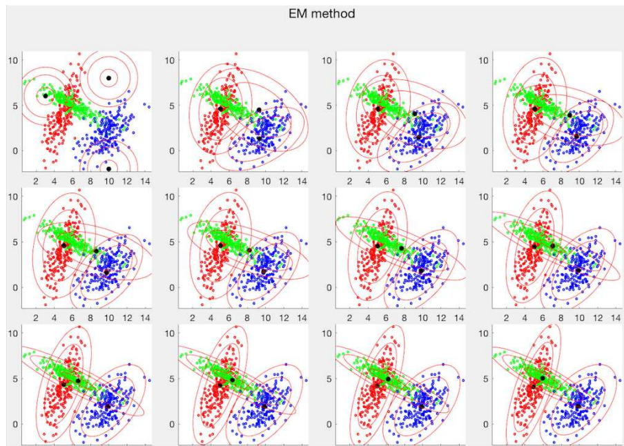
Figure 15.6 Clustering by Gaussian Mixture Model (first 12 iterations)
