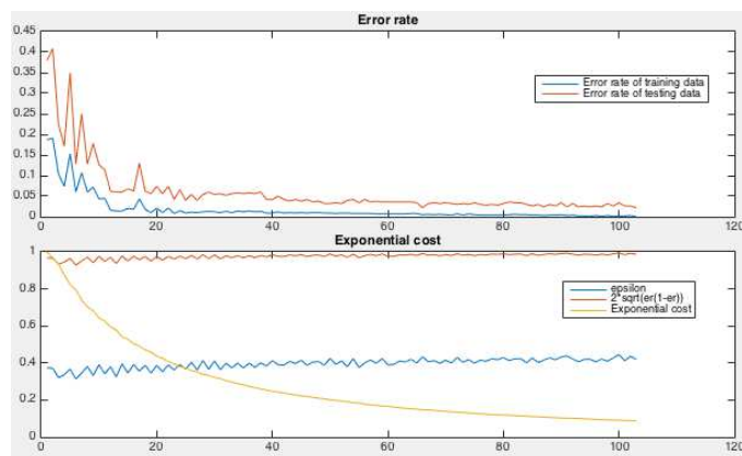
Figure 13.16 Progress of Iterative Training of AdaBoost
