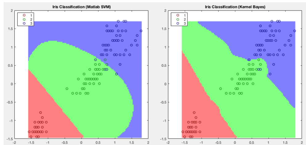
Figure 14.19 Comparison of kernel Bayes and SVM applied to iris data
