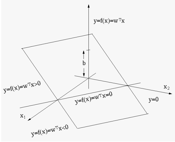
Figure 5.1 Linear Regression as a Binary Classifier
