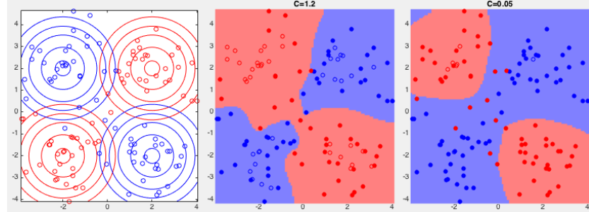
Figure 14.8 Classification of XOR Dataset by SVM Based on SMO
