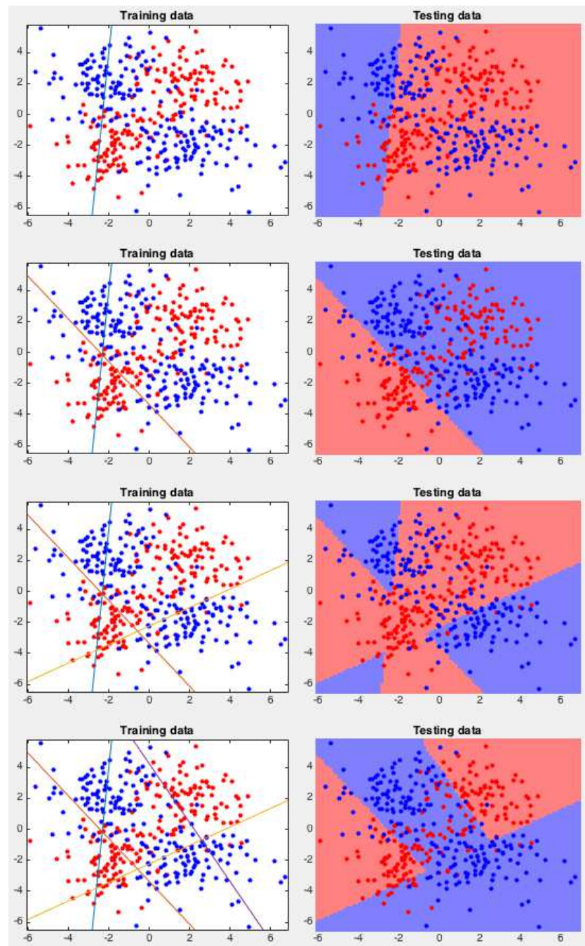
Figure 13.13 Classification by AdaBoost on XOR Dataset (early iterations)
