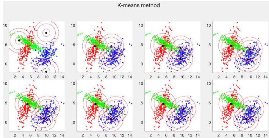
Figure 15.5 Clustering by K-Means Method (first 8 iterations)
