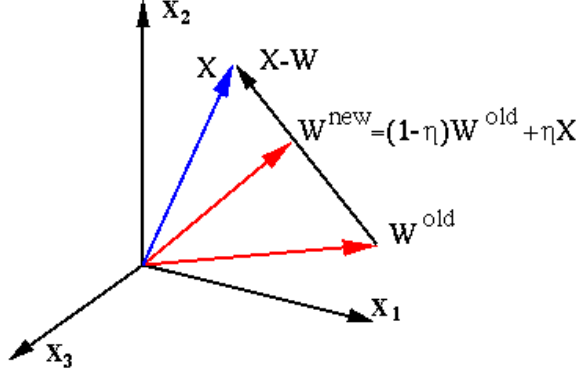
Figure 19.1 Modification of Weight Vector of the Winner
