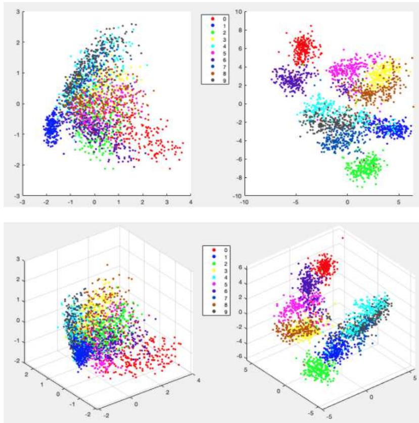
Figure 11.12 Visualization of 256-D dataset by the PCA (left) and tSNE (right) methods
