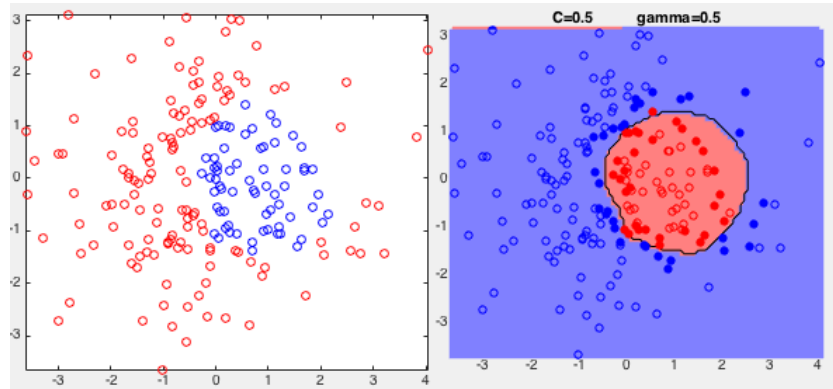
Figure 14.9 Example of Classification by SMO
