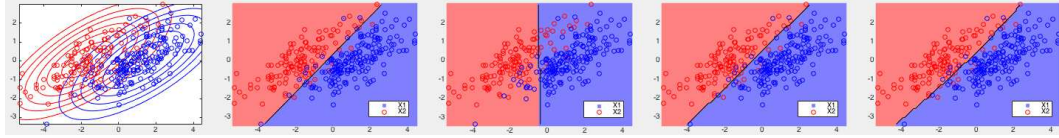
Figure 14.12 Example 1 of Kernelized Bayes Classifier
