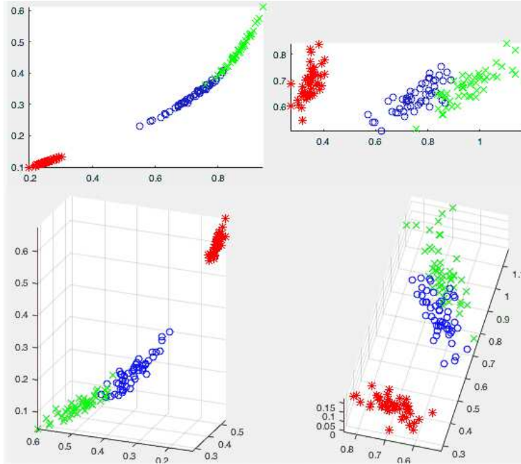
Figure 18.10 Autoencoder (Left) vs. KLT (right) for Dimension Reduction
