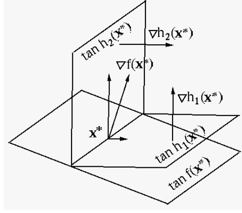
Figure 3.2 Derivation of Lagrange Function
