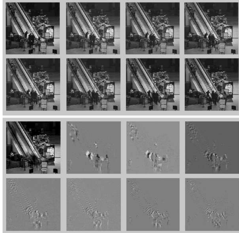
Figure 10.8 Eight frames of a video before (top) and after (bottom) the KLT
