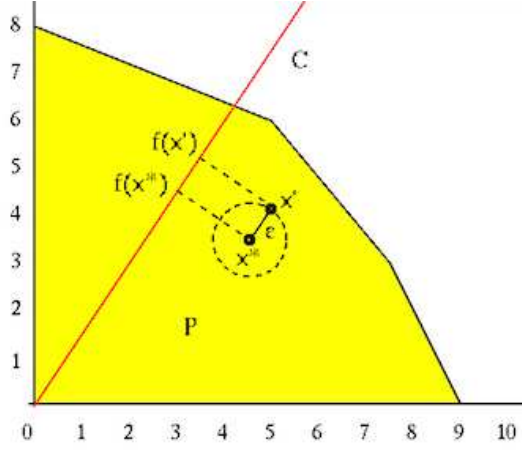
Figure 3.6 Fundamental Theorem of Linear Programming
