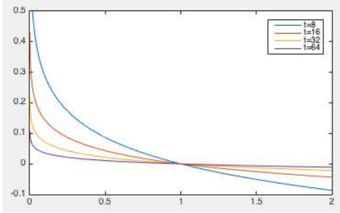
Figure 3.9 Logarithmic Barrier Function
