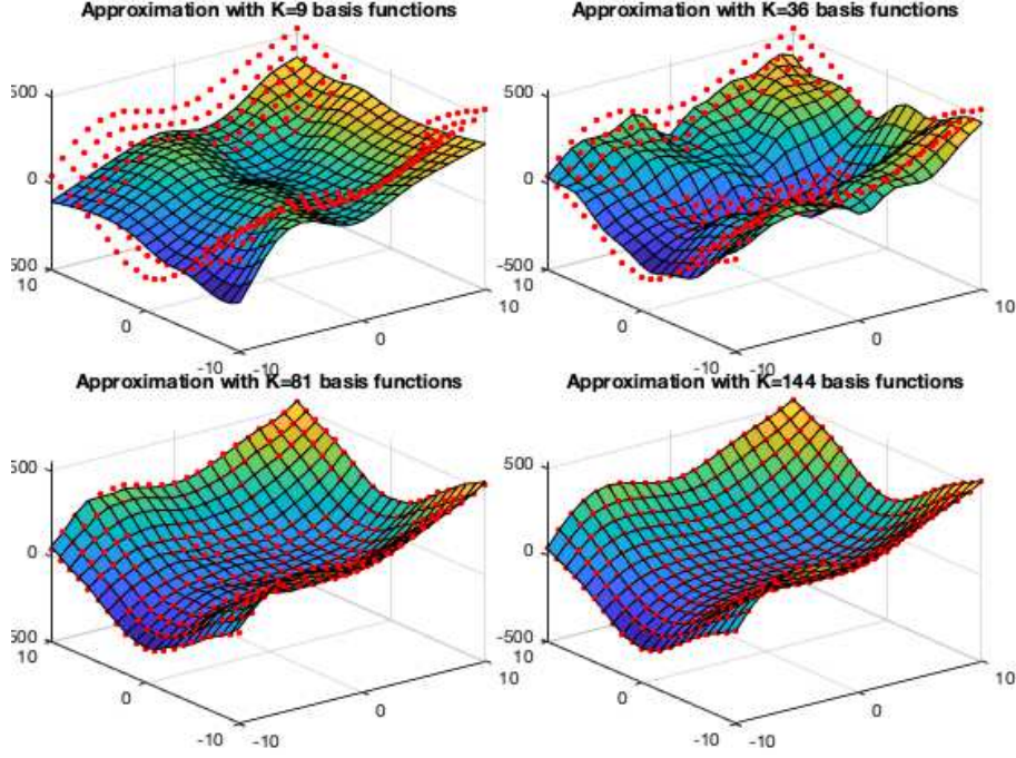
Figure 5.21 Regression based on Sigmoid Basis
