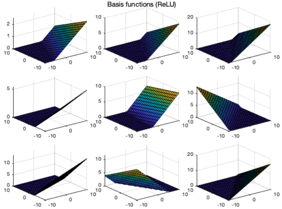
Figure 5.22 ReLU Basis for 2-D Regression
