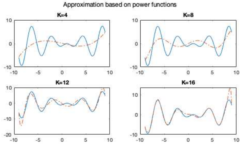
Figure 5.12 Regression based on Power Basis
