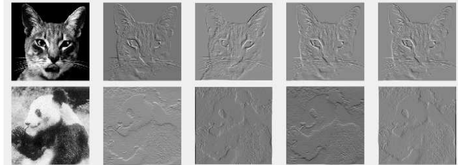
Figure 18.16 Directional Filtering
