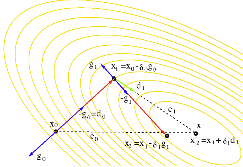
Figure 2.13 Conjugate Gradient Descent
