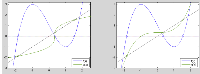
Figure 1.8 Example 1.5, plots of g_1(x) (left) and g_2(x) (right)
