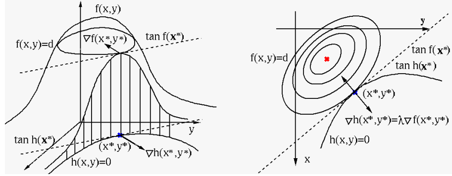
Figure 3.1 Equality Constrained Optimization of Function f(x, y)
