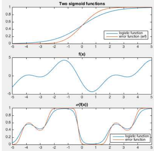
Figure 7.3 Convert Regression Function to Probability
