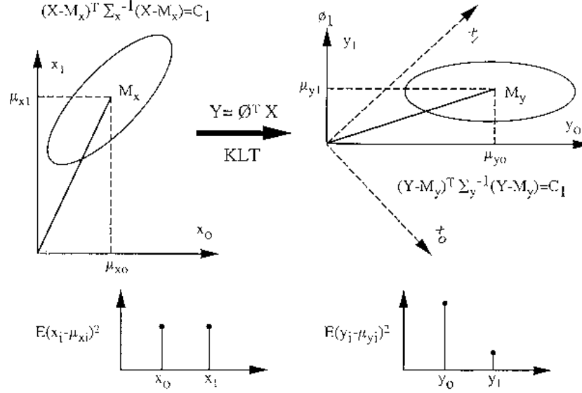
Figure 10.3 Standardization of ellipsoids by the KLT
