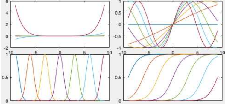
Figure 5.11 Basis Functions for Regression
