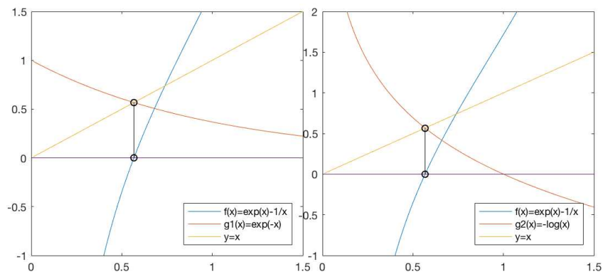
Figure 1.5 Example 1.3: Iteration converges for g(x) (left) but diverges for g'(x) (right)
