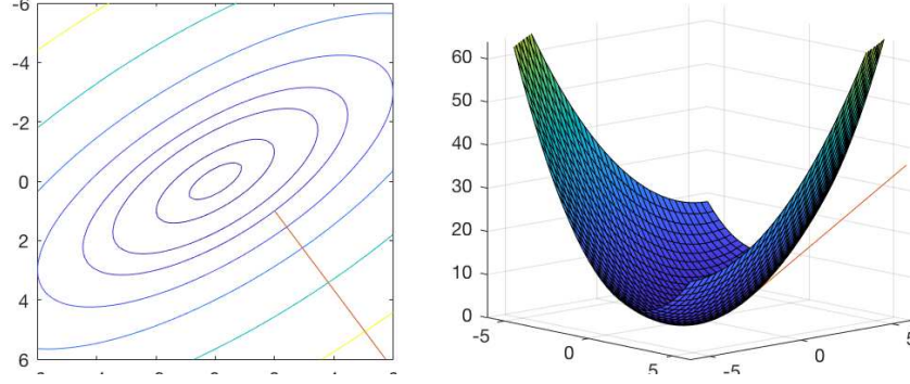
Figure 2.3 Gradient of a Quadratic Surface
