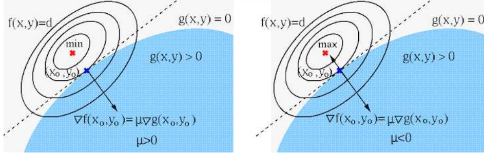
Figure 3.3 Inequality Constrained Optimization of f(x, y)
