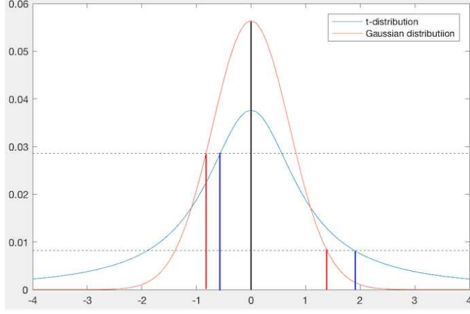
Figure 11.11 The t-distribution compared to the Gaussian distribution
