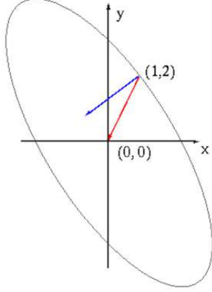
Figure 2.4 Comparison of Gradient Descent and Newton's Method
