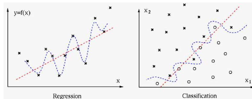
Figure 4.4 Under and Overfitting in Regression and Classification
