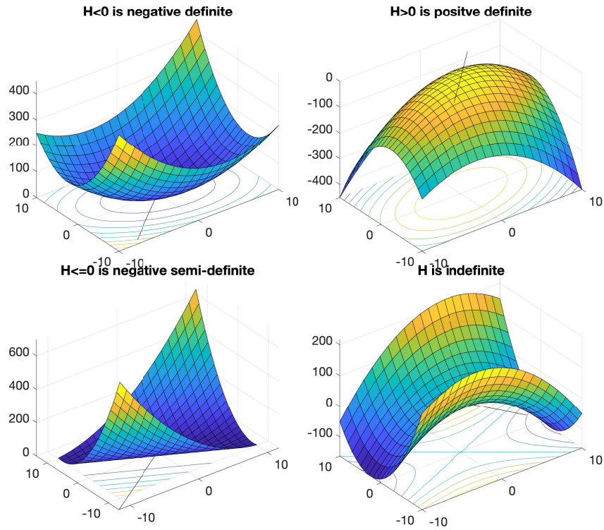
Figure 2.2 Quadratic Surfaces
