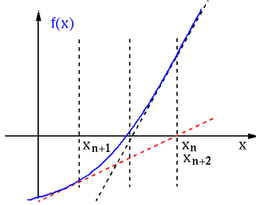
Figure 1.11 Oscillation
