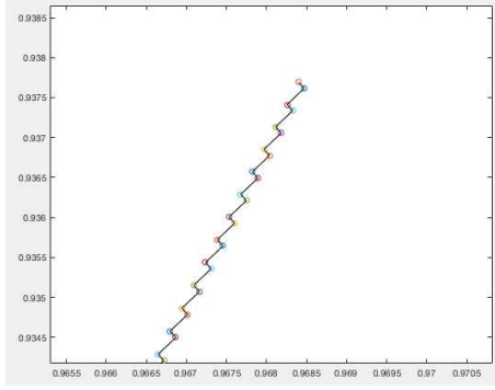
Figure 2.8 Search Path of the Gradient Descent (zoomed-in)
