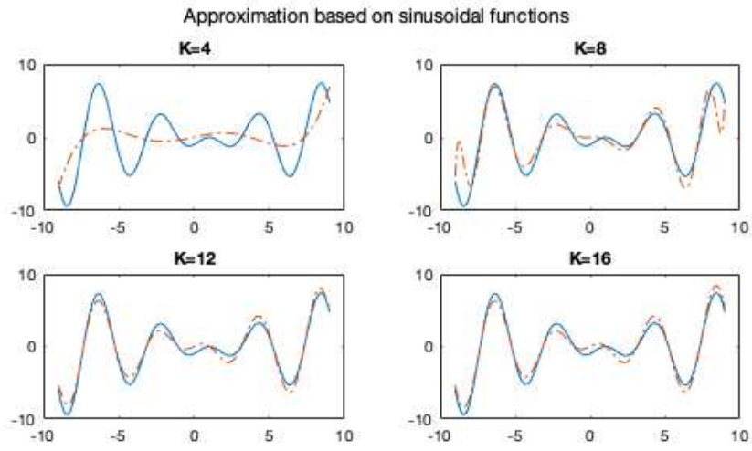
Figure 5.13 Regression based on Sinusoidal Basis
