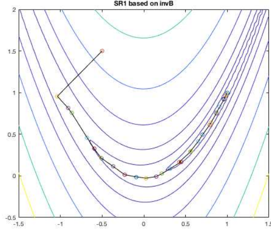
Figure 2.9 Search Path of SR1 based on \mathbf{B}^{-1}
