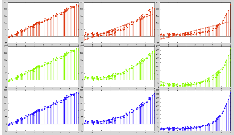
Figure 6.1 Nonlinear Regression with Multiple Datasets and Models (1-D)
