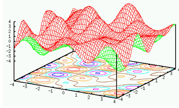
Figure 17.5 Energy Landscape
