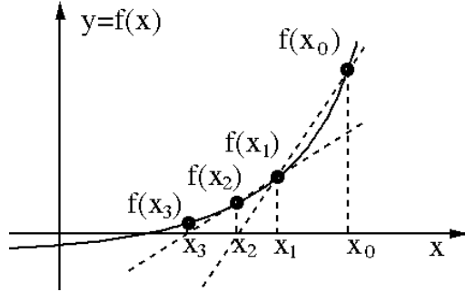
Figure 1.3 The Secant Method
