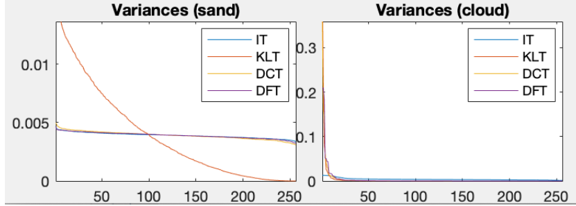
Figure 10.6 Energy compaction and redistribution by the KLT
