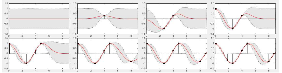
Figure 8.2 Gaussian Process Regression with Varying Data Points
