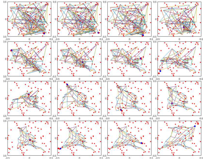
Figure 19.7 Iterative Learning of SOM (First 16 Iterations)
