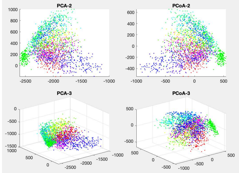
Figure 11.10 Visualization of the handwritten digits dataset based on both PCA and PCoA
