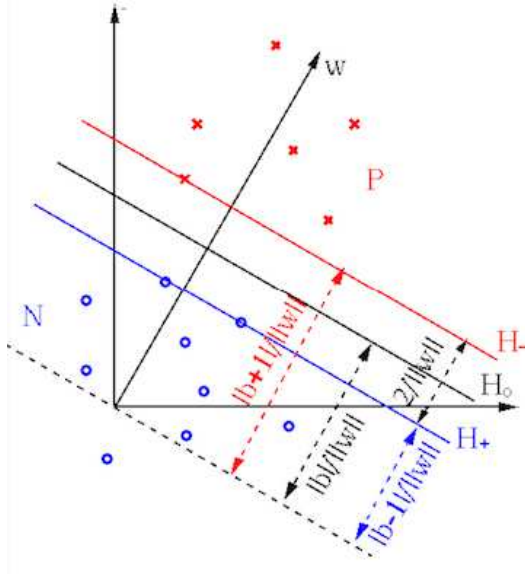
Figure 14.3 Decision Plane and Margin
