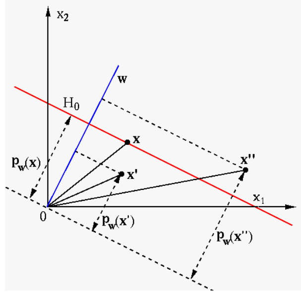
Figure 14.2 Decision Plane and Decision Margin
