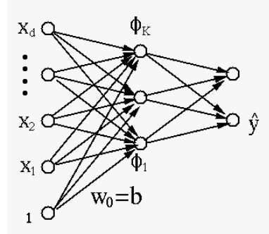
Figure 5.19 A Network Model for Regression
