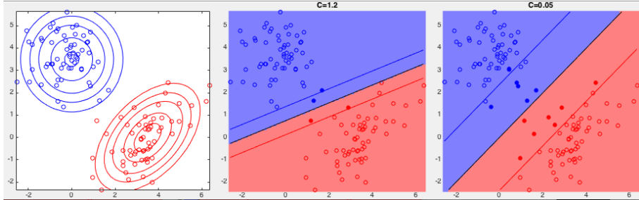
Figure 14.7 Classification by SVM Based on SMO
