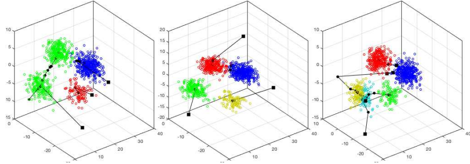
Figure 15.1 K-Means Clustering with K = 3 (left), K = 4 (middle), and K = 5 (right)
