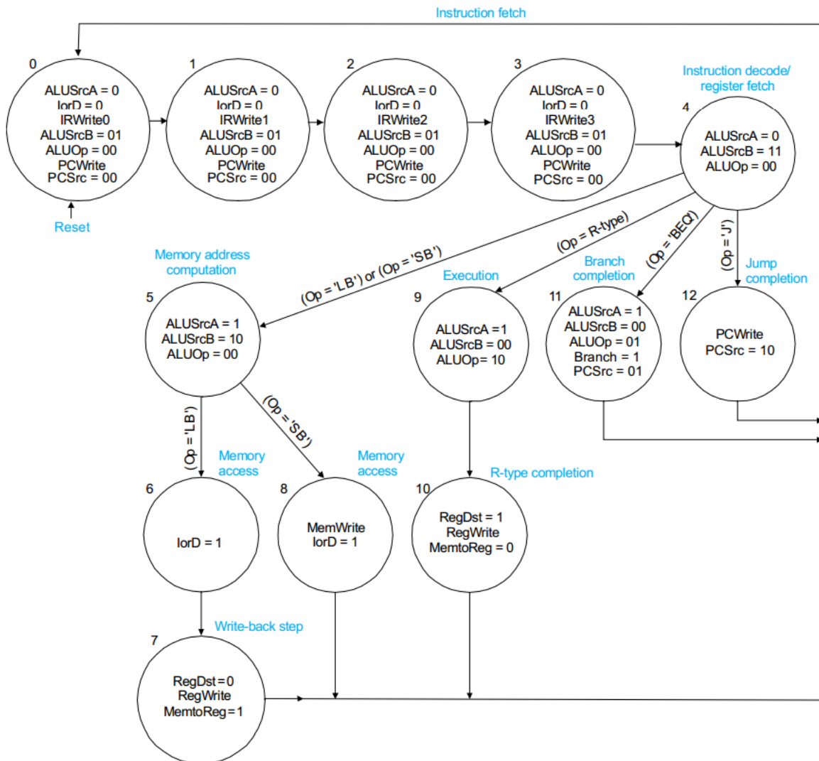
Figure 2: Controller FSM
